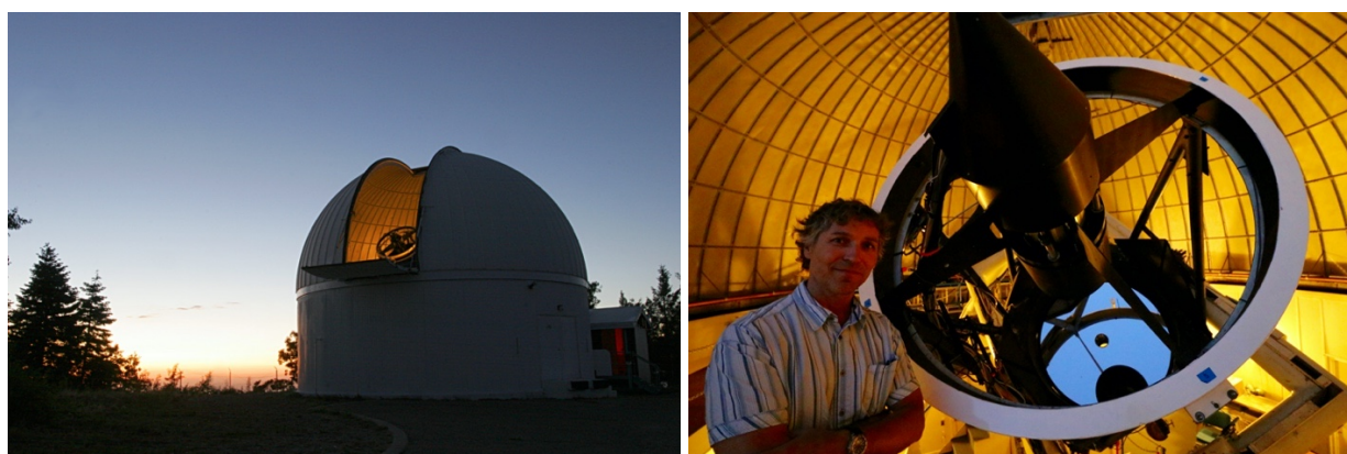
Figure 2 – The 1.5-m Catalina Sky Survey telescope on Mount Lemmon, MPC code G96.
