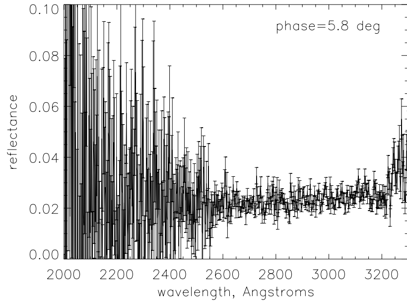
Interamnia Average
