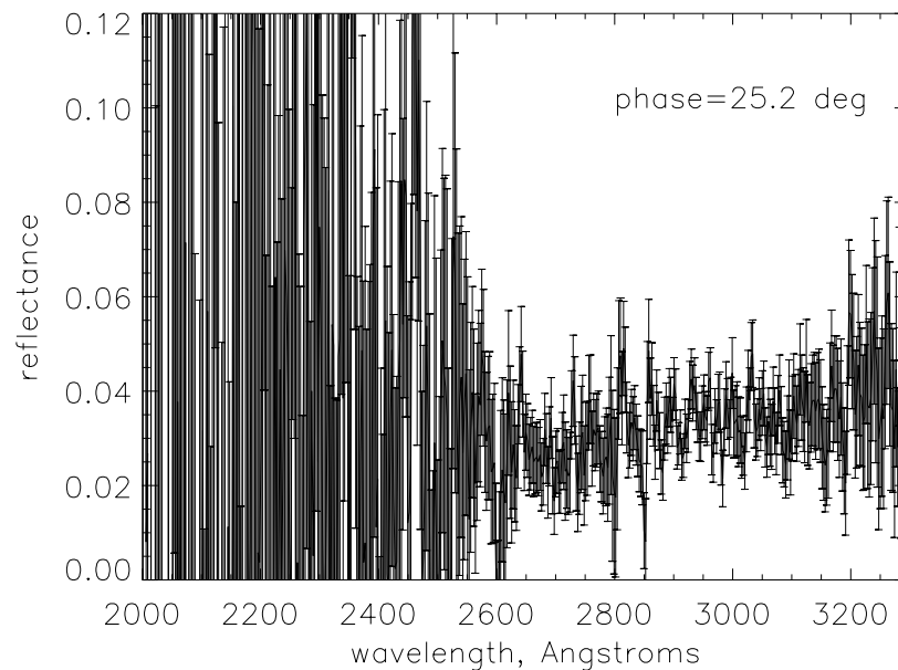
Massalia IUE LWR10612LL
