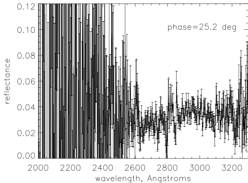
Massalia IUE LWR10598LL
