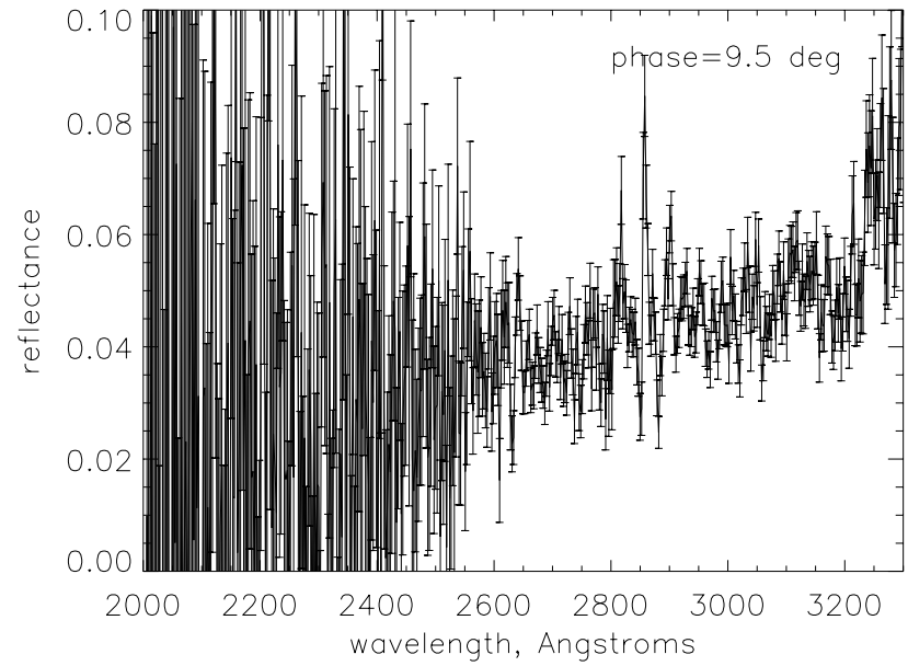
Irene IUE LWR07900LL
