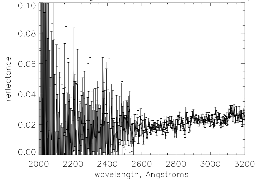
Juno Average (LWR05678LL, LWR05679LL)
