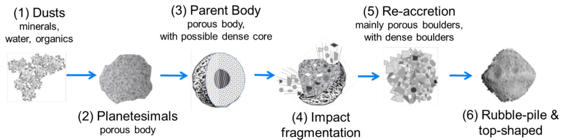
Extended Data Fig. 4 | A formation scenario of Ryugu from a porous parent body. (1) The formation started with fluffy dust in the solar nebula. (2) Porous planetesimals were formed by accretion of dust or pebbles. (3) The parent body of Ryugu might remain porous due to a low degree of consolidation. A clear boundary of the inner core is illustrated but a gradual increase of consolidation by depth could be expected. (4) Impact fragmentation of the parent body occurred. Some large fragments are the boulders on Ryugu. (5) Part of fragments were re-accreted to form Ryugu with porous boulders and sediments on the surface, with some dense boulders originated from the inner core. (6) Re-shape by rotation rate change to form a double top-shape.
