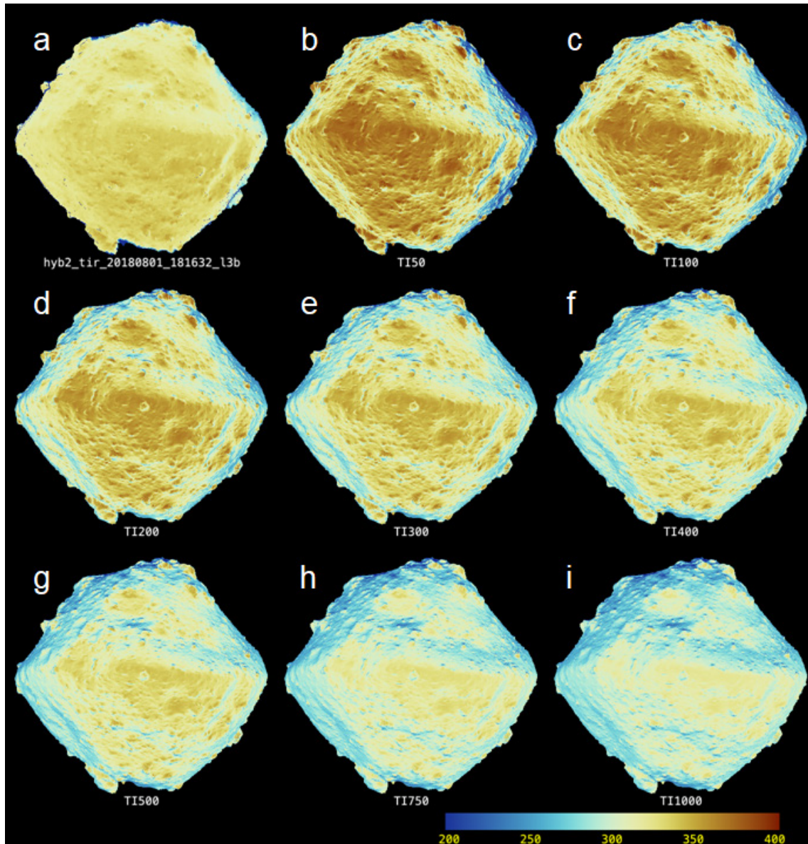
280 Fig. 2 | Comparison of a temperature plot on the 3D shape model with calculated images for thermal inertias from 50 to 1000 tui. a, A temperature plot in K on the asteroid Ryugu shape model (SHAPE_SFM_200k_v20180804), using the thermal image taken by TIR at 18:16:32 UTC on 1 Aug 2018 during the Mid-Altitude Observation Campaign. b-i, Calculated thermal images to be compared with the observation, b, assuming the uniform thermal inertia (TI) of 50 tui, c, TI of 100 285 tui, d, TI of 200 tui, e, TI of 300 tui, f, TI of 400 tui, g, TI of 500 tui, h, TI of 750 tui, and i, TI of 1000 tui. TI of 300 \pm 100 tui is most suitable to the observation.
