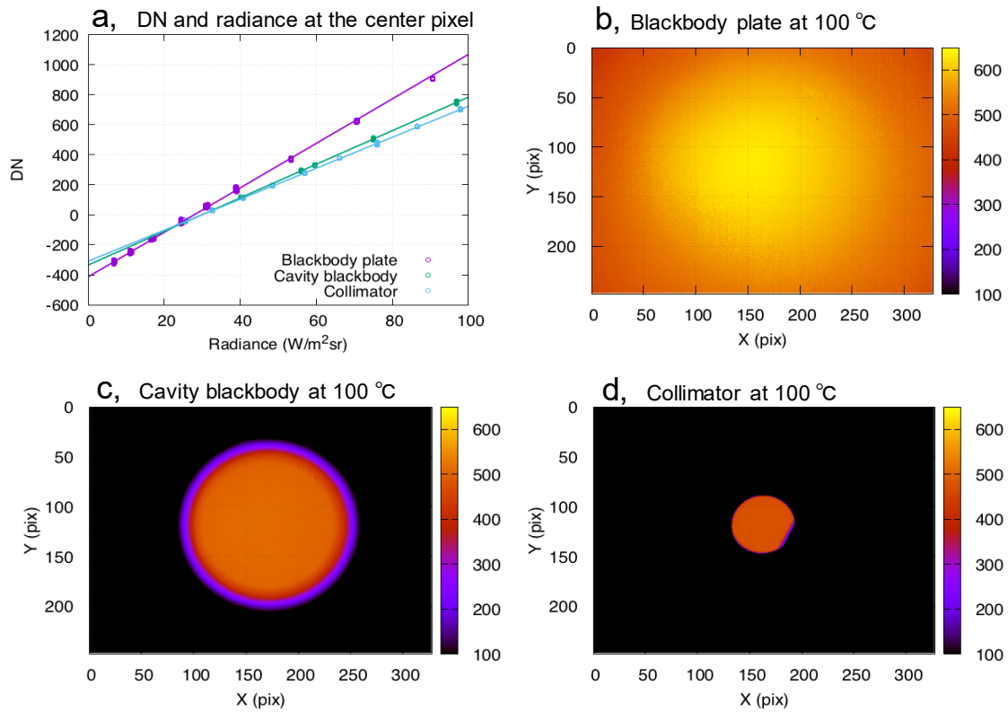
525 Extended Data Fig. 2 | Temperature calibration of TIR using multiple apparatuses. a , An example of TIR pixel response of a center pixel (164, 124) obtained by the ground-based calibration tests. The purple dots and line show the data for the blackbody plate and those linear regression. The blue and green dots show the data for the cavity blackbody and the collimator, respectively. b-d , Thermal images of TIR using the different apparatuses for the target of 100 °C : b , the blackbody plate (total area coverage), c , the cavity blackbody (simulation to Mid-Altitude), and d , the collimator (simulation to Home Position). 530
