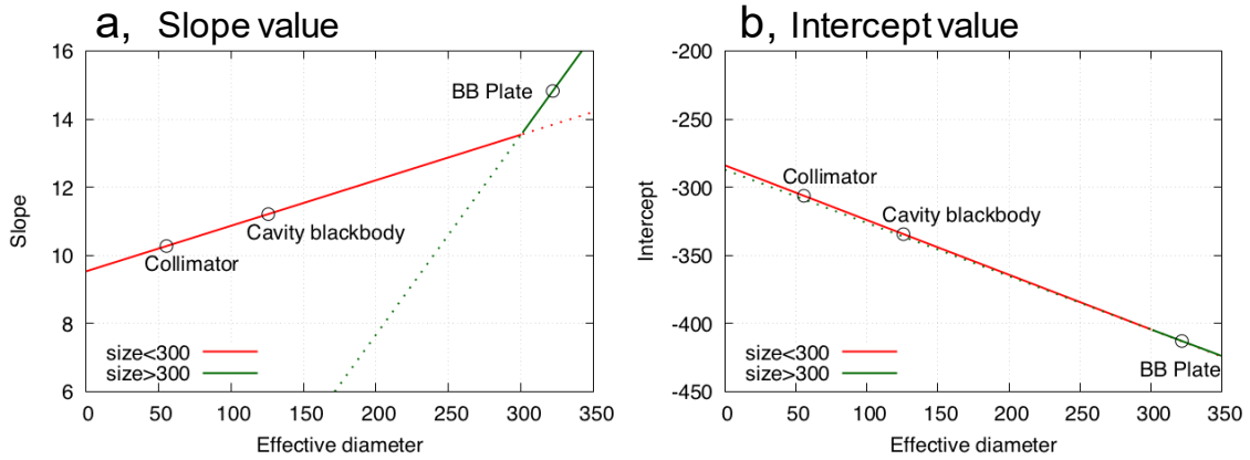
540 Extended Data Fig. 3 | Effective diameter dependence of the LUT for TIR calibration. This figures show the values of slope a and intercept b at the center pixel of (164, 124) in terms of the effective diameter D of the target. If D \leq 300 ( pixels ), the red lines are applied derived from the data of the collimator and the cavity blackbody sources. If 300 < D \leq 322 ( pixels ), the green lines are applied derived from the black body plate source.
