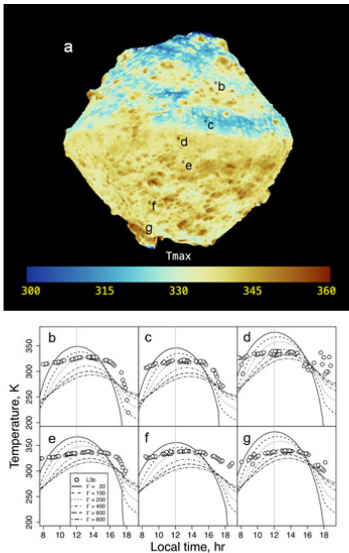
290 Fig. 3 | Maximum temperature distribution in during one rotation and the diurnal temperature profiles on Ryugu. a, Distribution of maximum temperature in K during one rotation on 1 August 2018 plotted on the Ryugu shape model (SHAPE_SFM_200k_v20180804). b-g, Diurnal temperature profiles by TIR observation (circles) and by thermal calculation (lines or dotted lines) with uniform thermal inertias from 20 to 800 tiu for each site of b to g in the plot a , respectively. The numbers in graph e are in tiu. The polygon IDs, the positions in longitude and latitude, 295 and the information of each site of b to g are shown in Extended Data Table 1.
