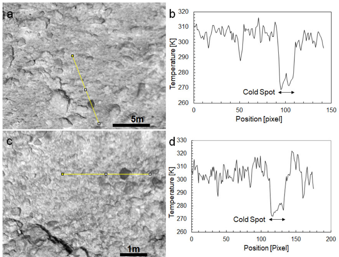
300 Fig. 4 | Cold spots discovered in the close-up thermal images. a, A close-up thermal image taken during the TD1-R1-A Campaign on 15 October 2018, at the solar distance of 1.28 au and the SPE angle of 10.6^\circ , at 13:34:44 UTC from the altitude of 78.8 m. b, The temperature profile on the yellow 305 line in the image (a), showing the “cold spot” boulder is identified. c, A close-up thermal image at 13:44:20 UTC at the altitude of 21.9 m. d, The temperature profile on the yellow line in the image (c), showing the “cold spot” boulder is identified. The surface is basically covered with boulders, and most of them have similar temperatures. The “cold spot” boulders show colder temperatures by more than 20 K, indicating dense and consolidated boulders with higher thermal inertia.
