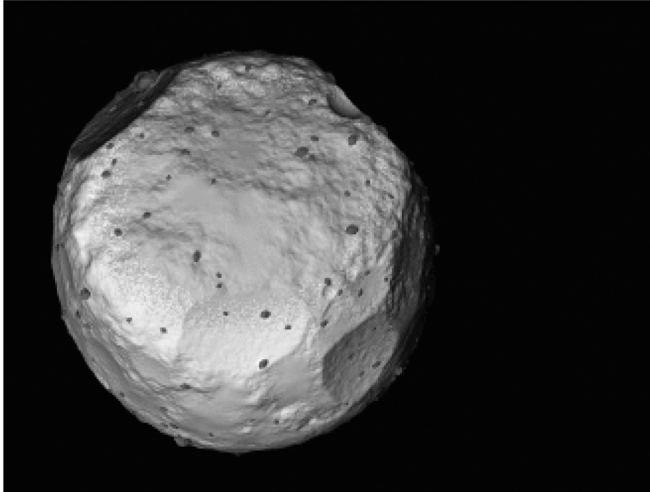
Extended Data Fig.1 | An expected thermal image of asteroid Ryugu before arrival. An example of the thermal image of the asteroid reference model “Ryugoid” produced by the Hayabusa2 Landing Site Selection Data Preparation team shows the surface covered with granular regolith (thermal inertia = 300 tiu) and dense boulders (thermal inertia =1600 tiu), and most of boulders are identified as “cold spots”.
