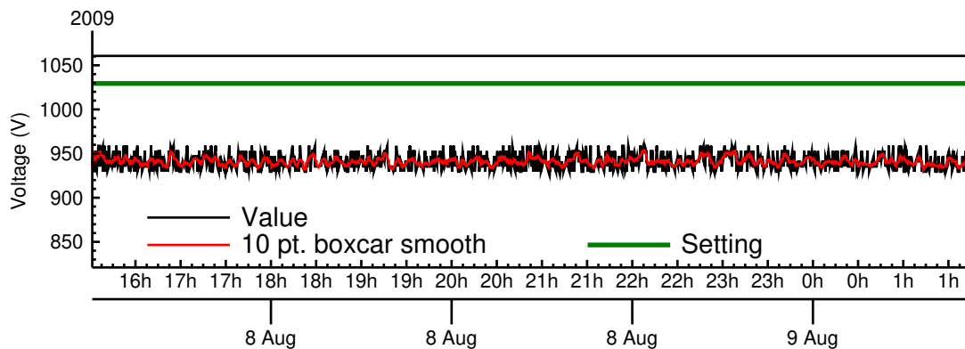
HVPS3 (+Y)
