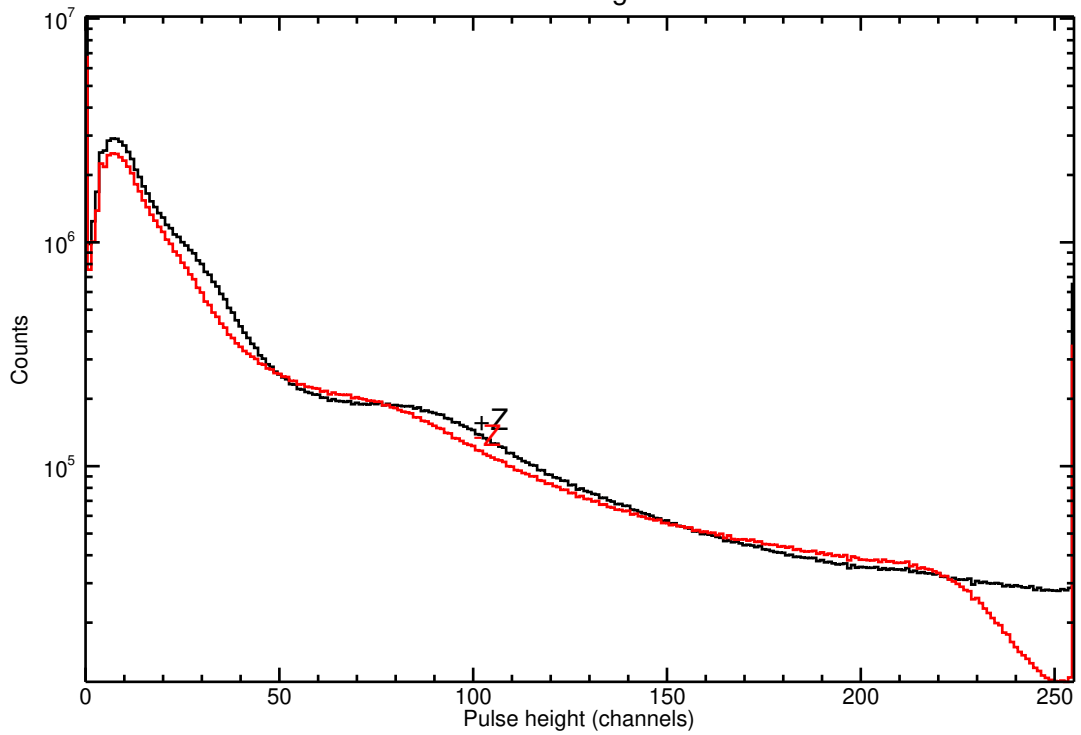
CAT1 histograms
