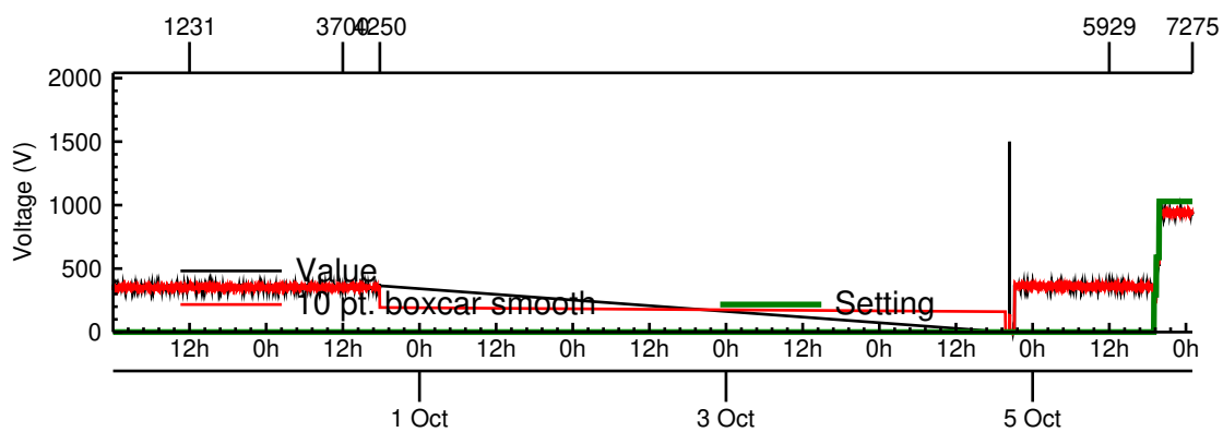
HVPS3 (+Y)
