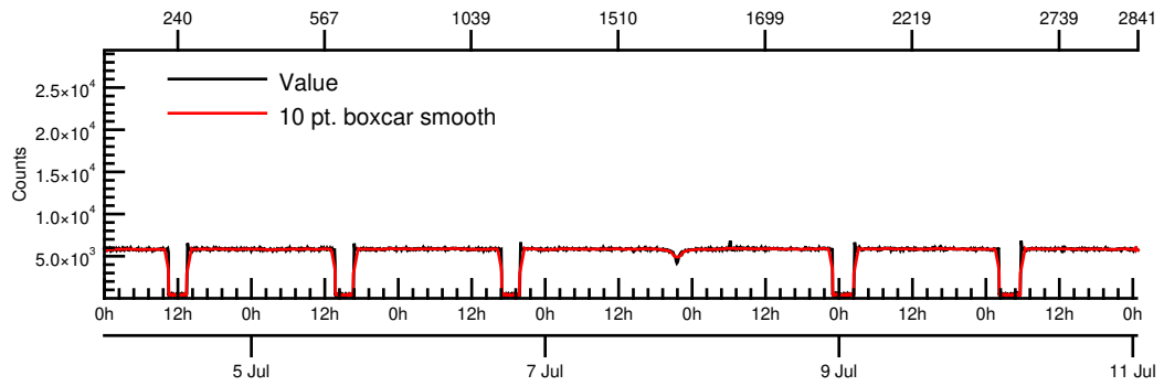
Multiple-crystal CZT events
