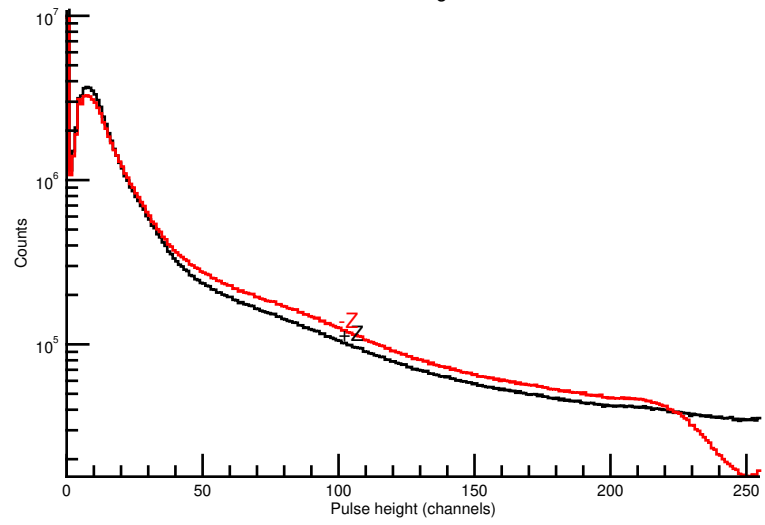
CAT1 histograms
