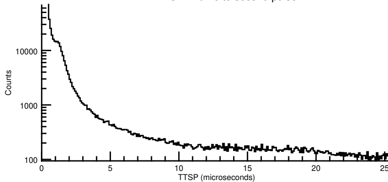
-Z BLP CAT4 time to second pulse
