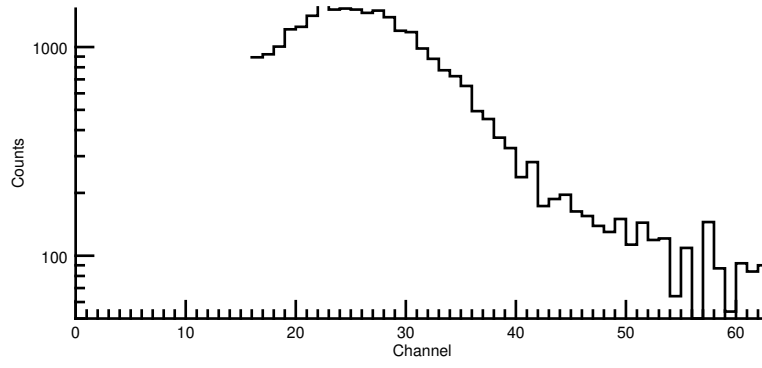
+Y BLP CAT4 time to second pulse
