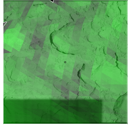
Figure 615: ST_2539451609_v.fits
