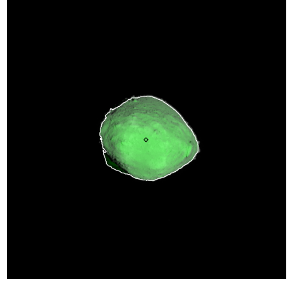
Figure 471: ST_2424173388_v.fits
