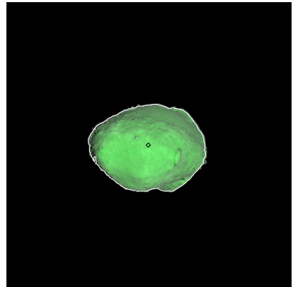
Figure 351: ST_2421314393_v.fits
