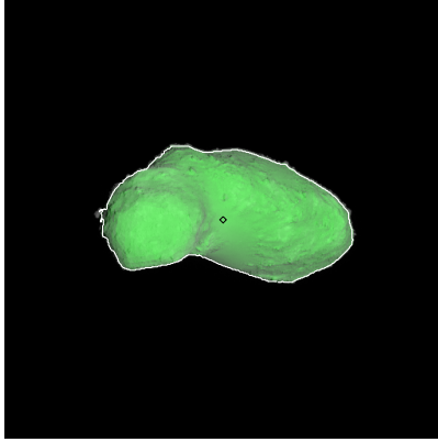
Figure 425: ST_2423288676_v.fits
