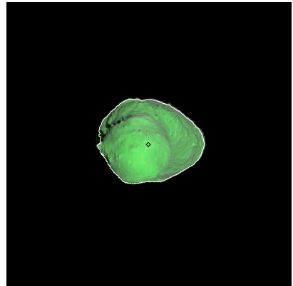
Figure 441: ST_2423419728_v.fits
