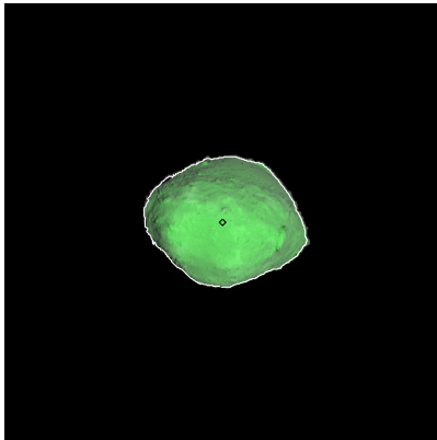
Figure 467: ST_2424140605_v.fits
