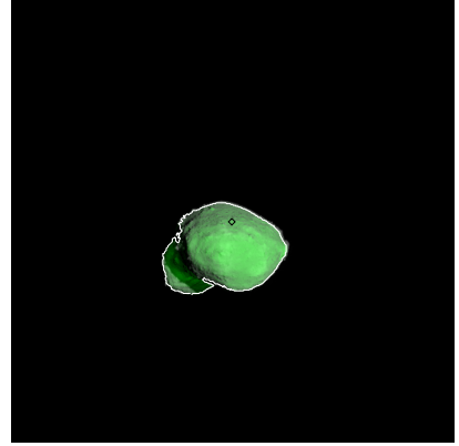
Figure 192: ST_2413048952_v.fits
