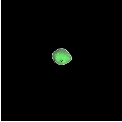
Figure 118: ST_2403227299_v.fits
