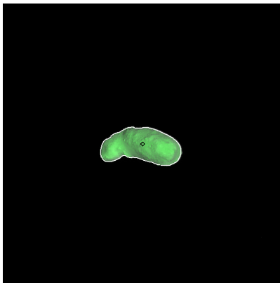
Figure 59: ST_2393695526_v.fits
