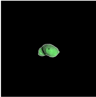
Figure 41: ST_2393557279_v.fits
