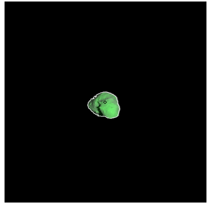
Figure 78: ST_2395584204_v.fits
