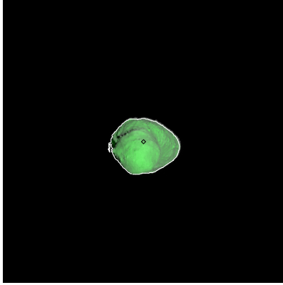
Figure 127: ST_2409469968_v.fits
