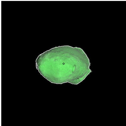
Figure 349: ST_2421298010_v.fits
