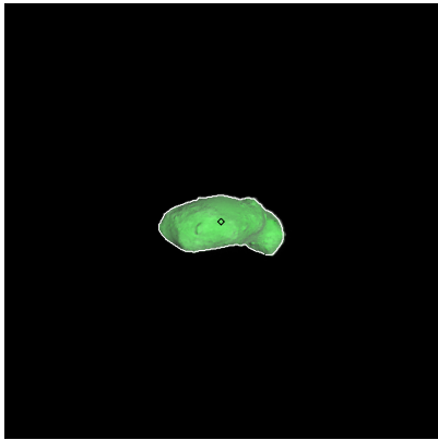
Figure 103: ST_2403006498_v.fits
