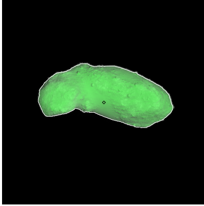
Figure 254: ST_2417597632_v.fits
