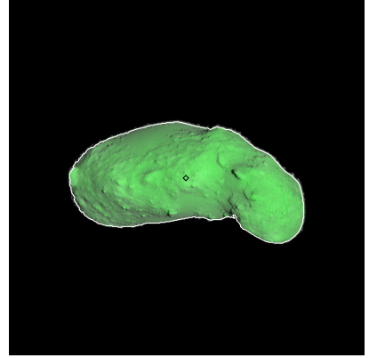
Figure 300: ST_2420896633_v.fits
