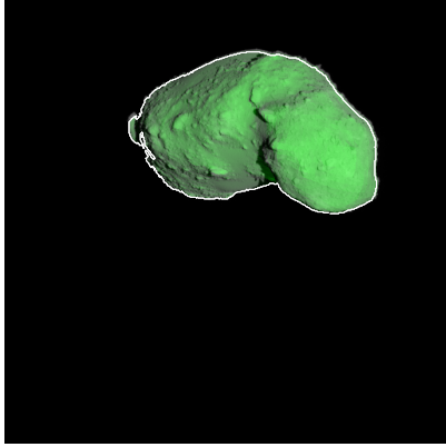
Figure 271: ST_2419381121_v.fits
