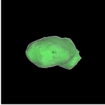
Figure 343: ST_2421248876_v.fits
