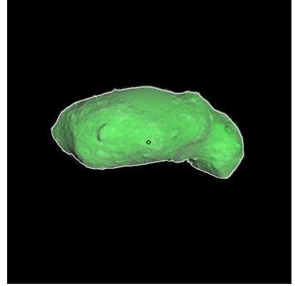
Figure 264: ST_2418699769_v.fits
