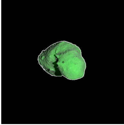
Figure 452: ST_2423509836_v.fits
