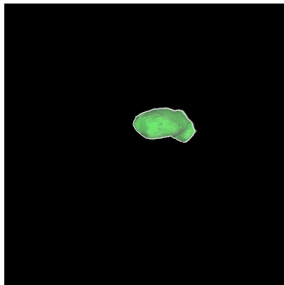
Figure 16: ST_2371015429_v.fits
