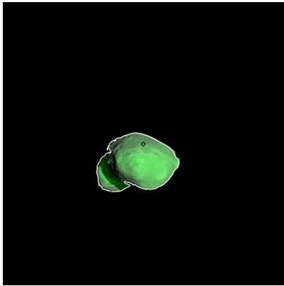
Figure 193: ST_2413056637_v.fits
