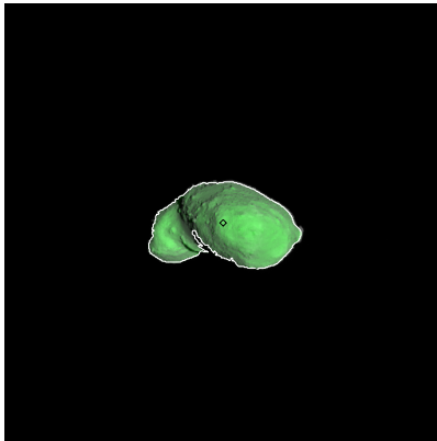
Figure 143: ST_2410330195_v.fits
