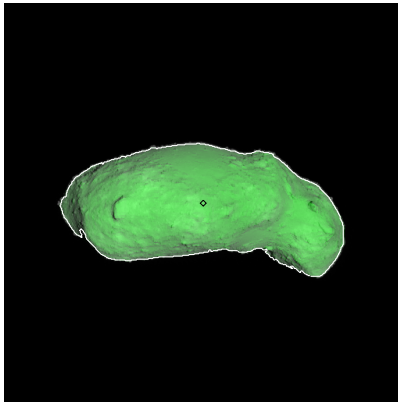
Figure 323: ST_2421085059_v.fits
