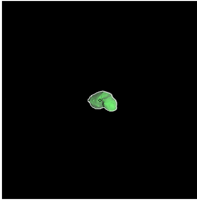
Figure 1: ST_2367722441_v.fits
