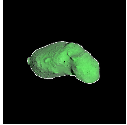
Figure 291: ST_2420822891_v.fits
