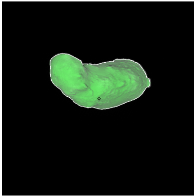
Figure 536: ST_2458574873_v.fits
