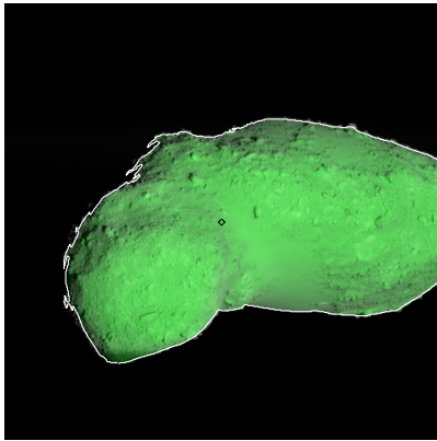
Figure 580: ST_2490253205_v.fits
