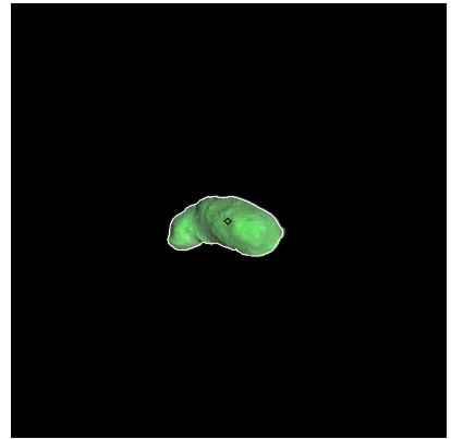
Figure 51: ST_2393634079_v.fits
