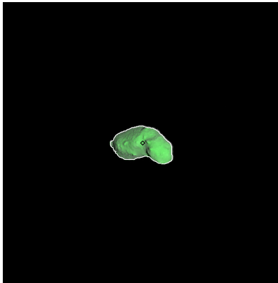
Figure 89: ST_2395676355_v.fits
