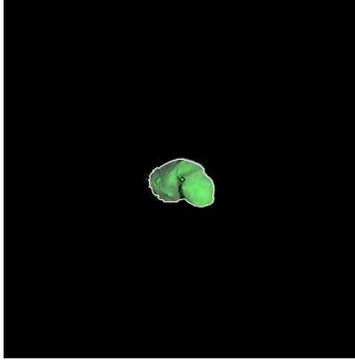
Figure 83: ST_2395630278_v.fits
