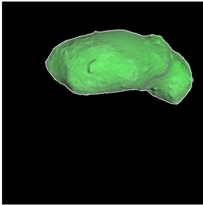
Figure 275: ST_2419753902_v.fits
