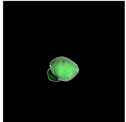
Figure 189: ST_2413025897_v.fits
