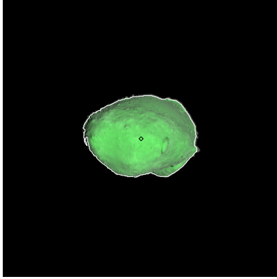
Figure 461: ST_2424091455_v.fits
