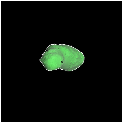
Figure 214: ST_2414976721_v.fits
