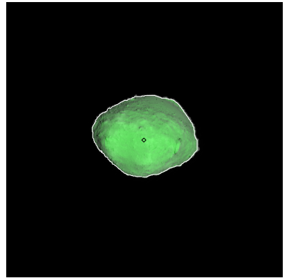
Figure 465: ST_2424124238_v.fits
