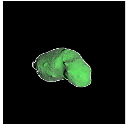
Figure 501: ST_2426360671_v.fits
