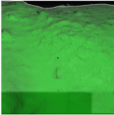
Figure 607: ST_2530286817_v.fits
