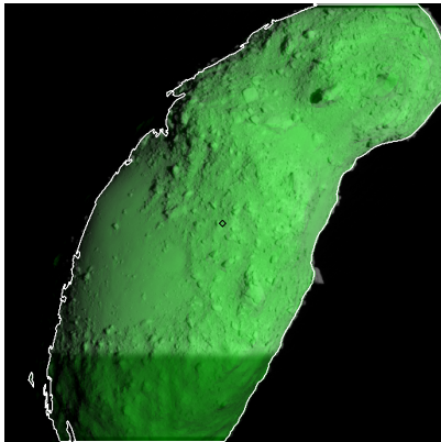
Figure 565: ST_2480981469_v.fits
