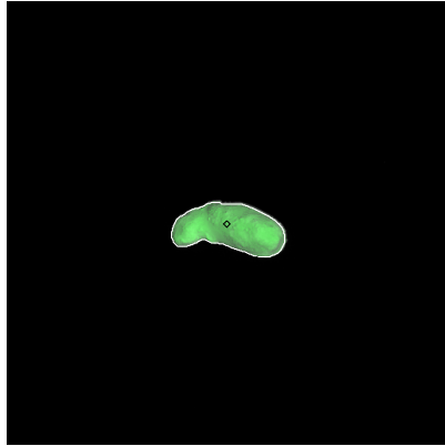
Figure 10: ST_2370353993_v.fits
