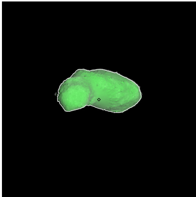
Figure 205: ST_2414907605_v.fits
