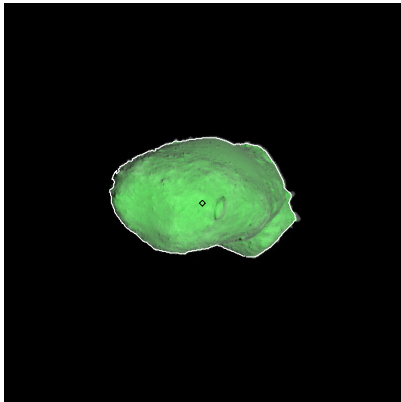
Figure 457: ST_2424058721_v.fits
