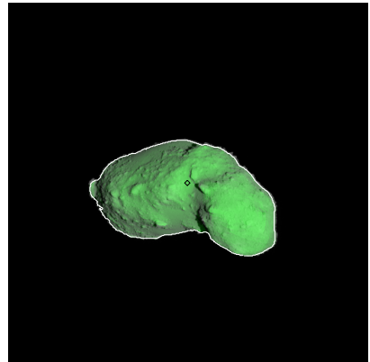
Figure 504: ST_2426385246_v.fits
