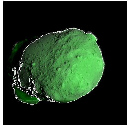
Figure 567: ST_2481442195_v.fits
