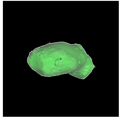
Figure 339: ST_2421216109_v.fits
