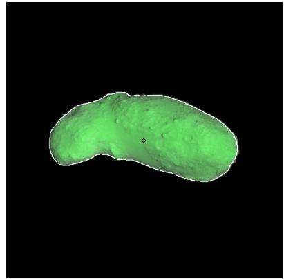
Figure 402: ST_2423092092_v.fits
