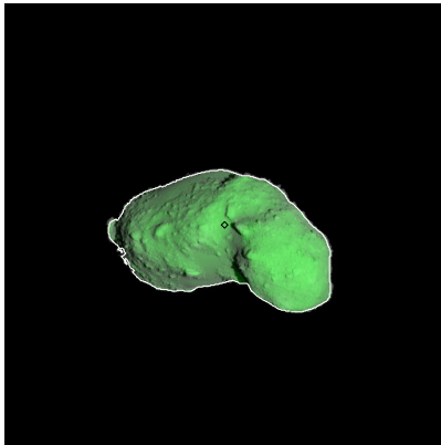
Figure 503: ST_2426377038_v.fits
