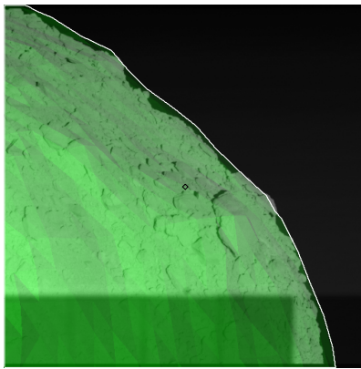
Figure 617: ST_2539482843_v.fits
