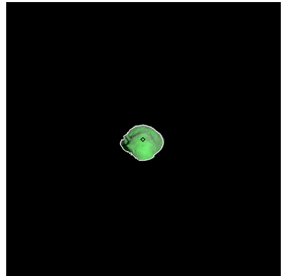
Figure 72: ST_2395538127_v.fits
