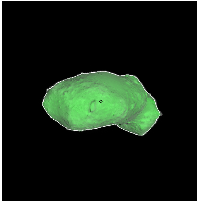
Figure 338: ST_2421207934_v.fits
