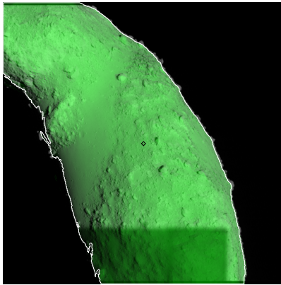
Figure 563: ST_2474731509_v.fits
