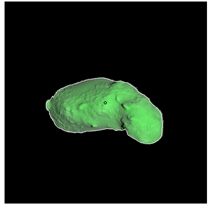
Figure 510: ST_2426434412_v.fits
