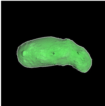
Figure 314: ST_2421011334_v.fits
