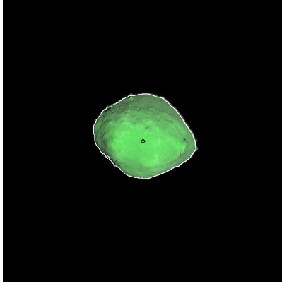
Figure 469: ST_2424157005_v.fits
