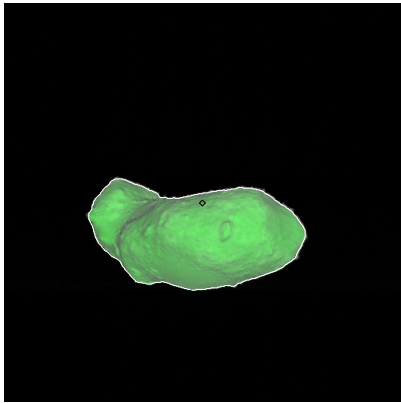
Figure 535: ST_2458542208_v.fits
