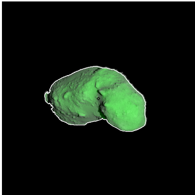
Figure 286: ST_2420781916_v.fits
