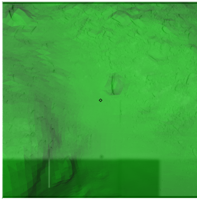
Figure 608: ST_2530292409_v.fits
