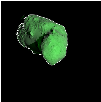
Figure 554: ST_2471012186_v.fits
