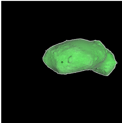
Figure 359: ST_2422575989_v.fits
