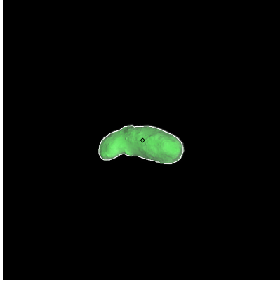
Figure 65: ST_2393741603_v.fits
