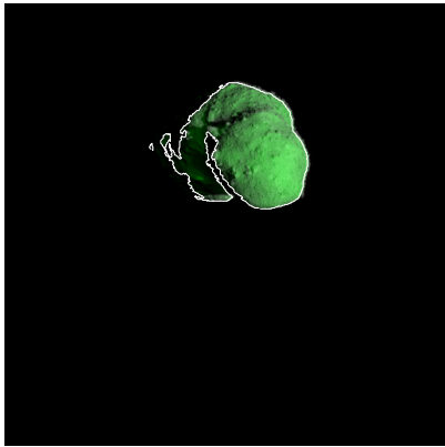
Figure 526: ST_2448576189_v.fits
