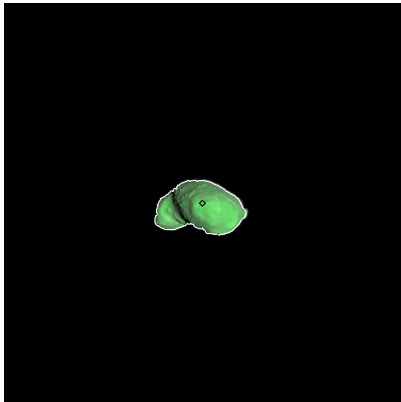
Figure 43: ST_2393572616_v.fits
