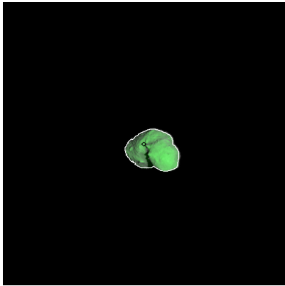
Figure 22: ST_2385835211_v.fits
