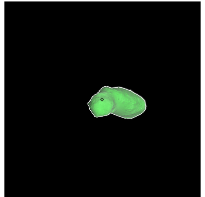
Figure 27: ST_2388426919_v.fits
