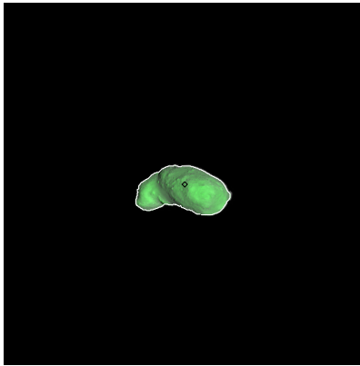
Figure 50: ST_2393626411_v.fits
