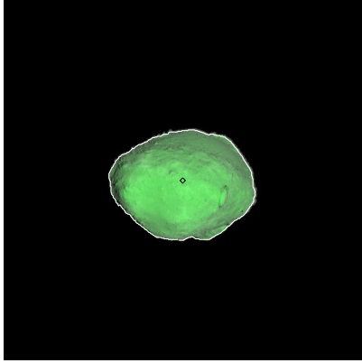
Figure 352: ST_2421322585_v.fits
