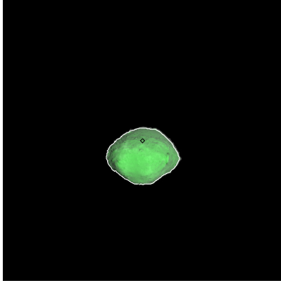
Figure 181: ST_2412964467_v.fits
