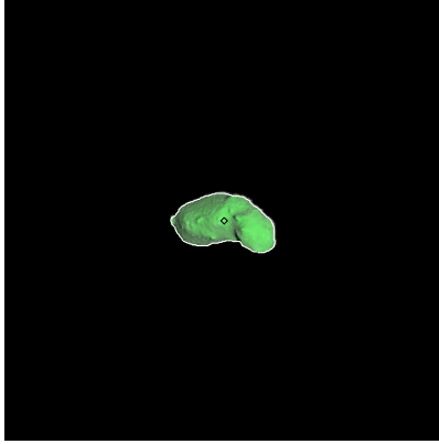
Figure 92: ST_2395699394_v.fits
