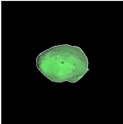
Figure 350: ST_2421306185_v.fits
