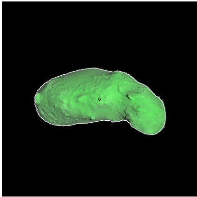
Figure 301: ST_2420904858_v.fits
