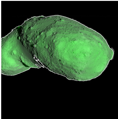
Figure 601: ST_2506656195_v.fits
