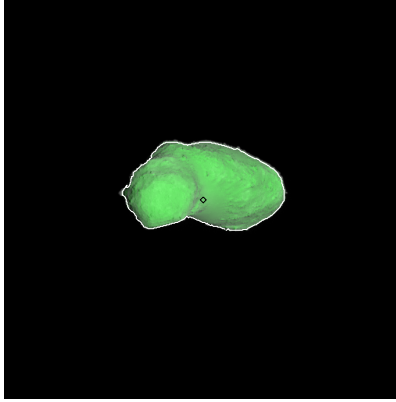
Figure 209: ST_2414938329_v.fits
