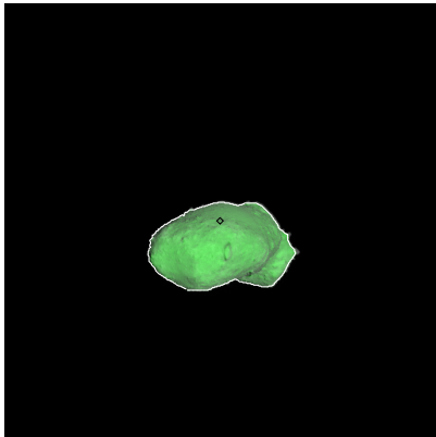
Figure 169: ST_2412872313_v.fits
