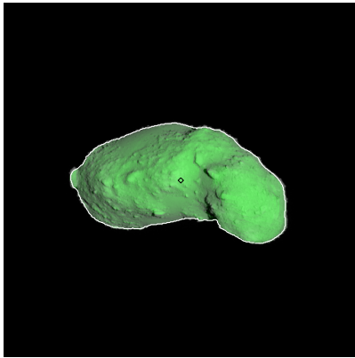
Figure 293: ST_2420839291_v.fits
