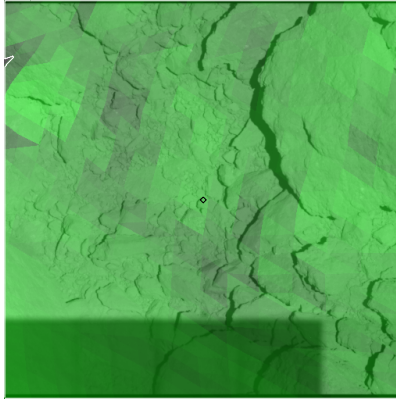
Figure 614: ST_2539444467_v.fits
