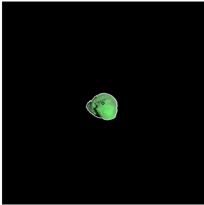
Figure 76: ST_2395568834_v.fits
