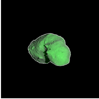
Figure 280: ST_2420732749_v.fits
