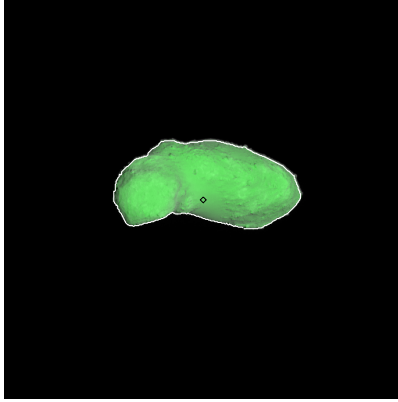
Figure 200: ST_2414869213_v.fits
