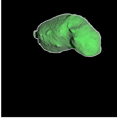
Figure 272: ST_2419389297_v.fits
