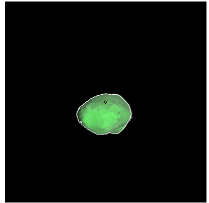
Figure 177: ST_2412933744_v.fits
