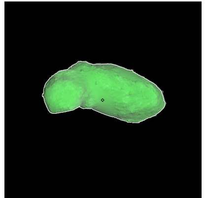
Figure 261: ST_2417651394_v.fits
