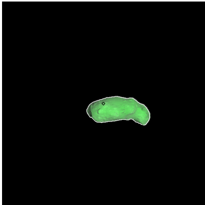
Figure 97: ST_2402929709_v.fits
