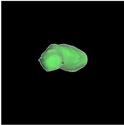
Figure 211: ST_2414953699_v.fits
