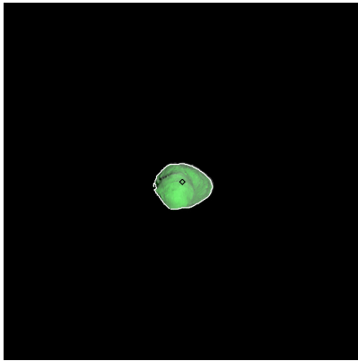
Figure 68: ST_2395507354_v.fits
