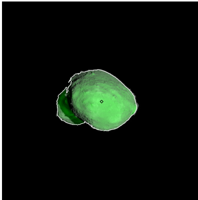
Figure 476: ST_2424214329_v.fits
