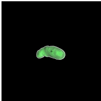
Figure 58: ST_2393687841_v.fits
