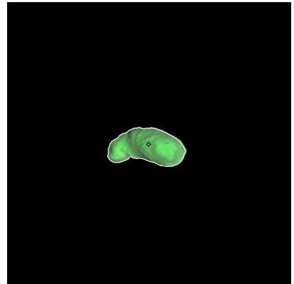
Figure 54: ST_2393657118_v.fits
