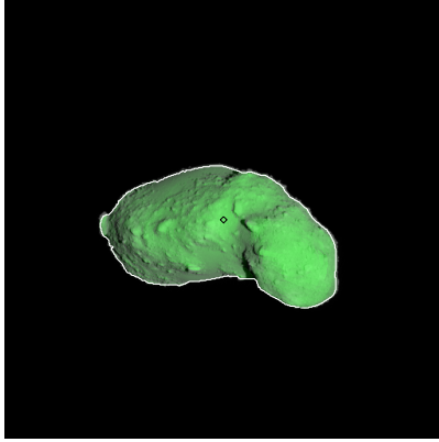
Figure 506: ST_2426401645_v.fits
