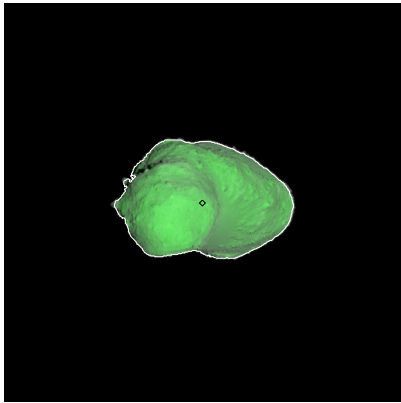
Figure 436: ST_2423378786_v.fits
