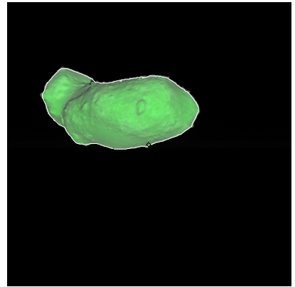
Figure 537: ST_2458929180_v.fits
