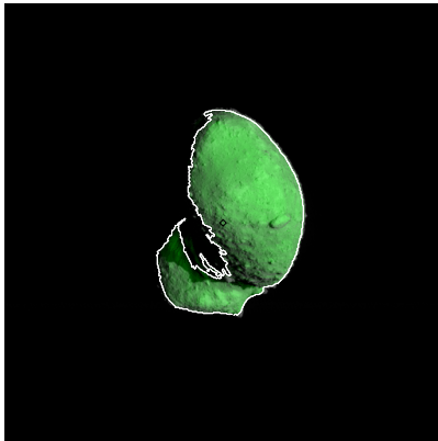
Figure 548: ST_2467348679_v.fits
