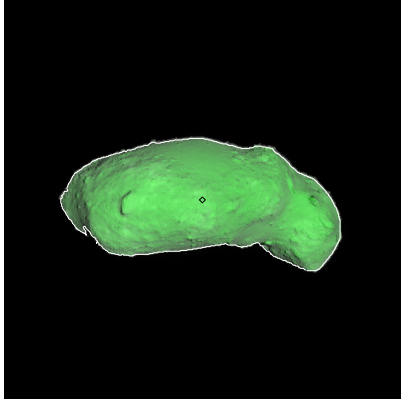
Figure 325: ST_2421101459_v.fits
