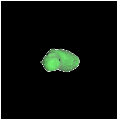
Figure 122: ST_2409393181_v.fits
