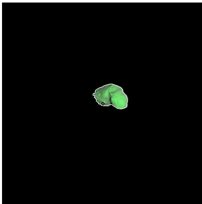
Figure 14: ST_2370593050_w.fits
