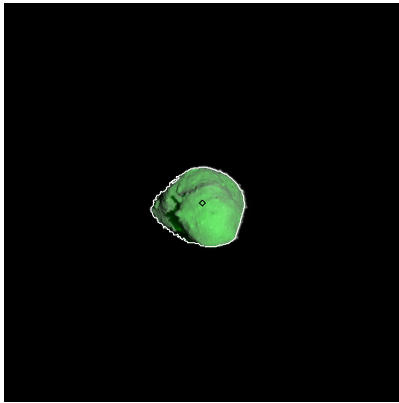
Figure 130: ST_2409516054_v.fits
