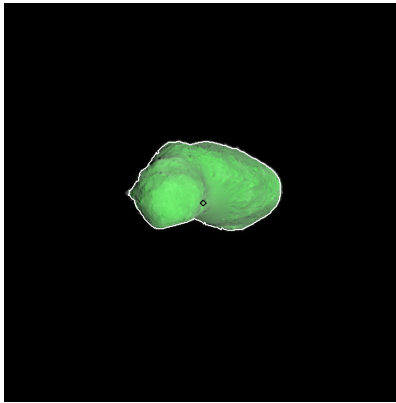
Figure 212: ST_2414961367_v.fits
