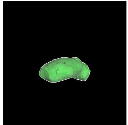
Figure 159: ST_2412795529_v.fits
