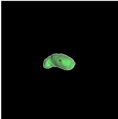
Figure 52: ST_2393641764_v.fits
