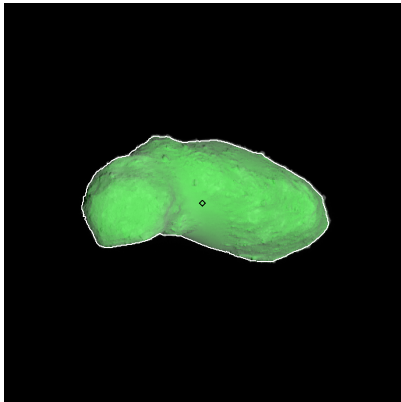
Figure 421: ST_2423255925_v.fits
