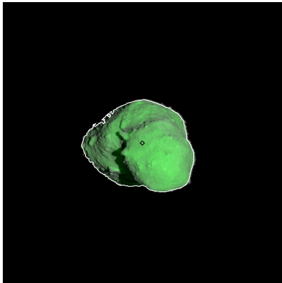
Figure 277: ST_2420708174_v.fits
