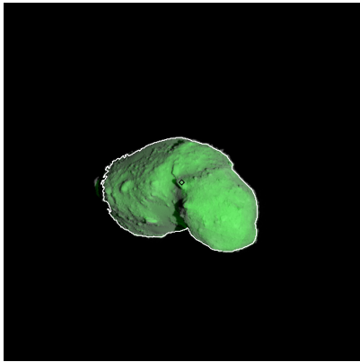
Figure 499: ST_2426344271_v.fits
