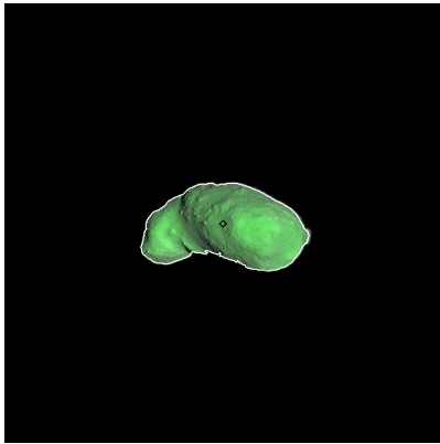
Figure 148: ST_2410368604_v.fits
