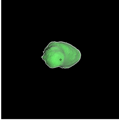
Figure 218: ST_2415007444_v.fits
