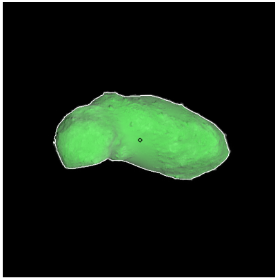
Figure 419: ST_2423239542_v.fits
