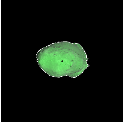
Figure 460: ST_2424083280_v.fits
