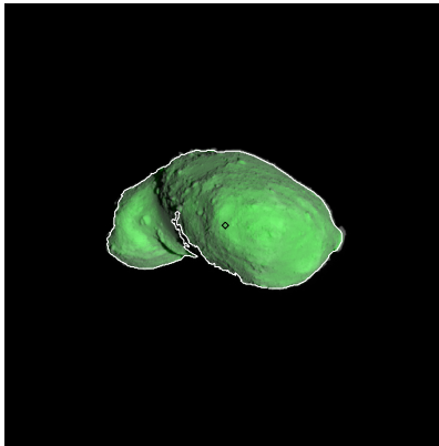
Figure 485: ST_2424288087_v.fits
