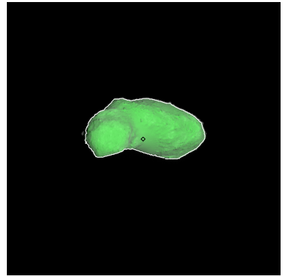
Figure 204: ST_2414899936_v.fits
