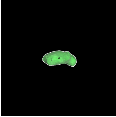
Figure 101: ST_2402987304_v.fits
