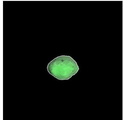
Figure 180: ST_2412956782_v.fits
