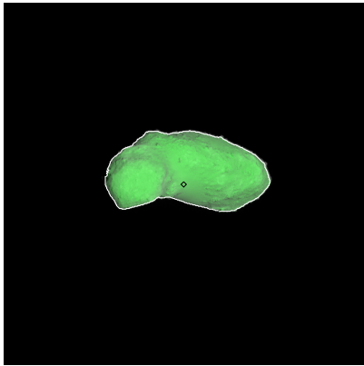
Figure 202: ST_2414884583_v.fits
