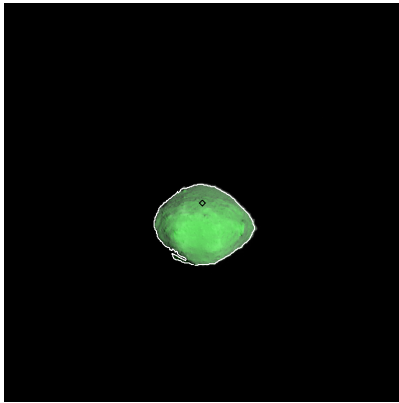
Figure 184: ST_2412987506_v.fits
