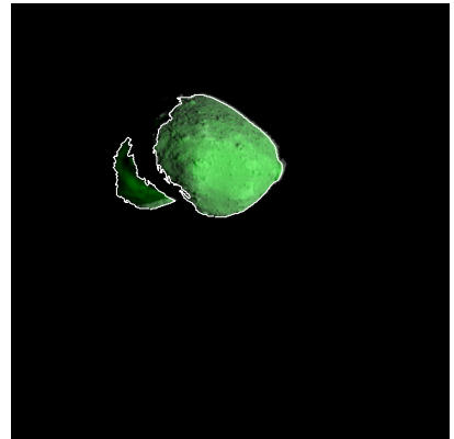
Figure 522: ST_2447904203_v.fits
