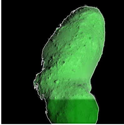
Figure 569: ST_2481929904_v.fits
