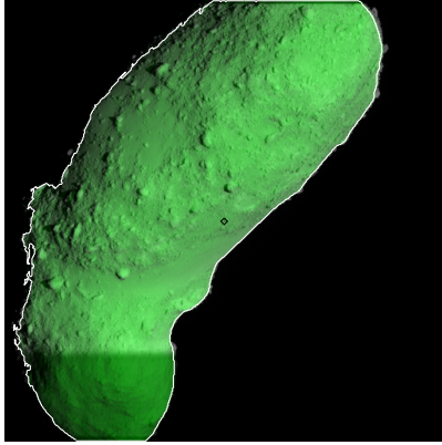
Figure 568: ST_2481672682_v.fits
