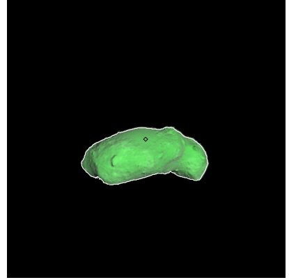
Figure 156: ST_2412734079_v.fits
