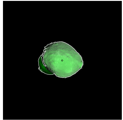
Figure 474: ST_2424197963_v.fits
