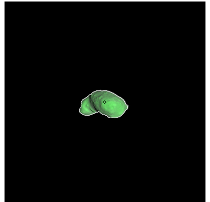
Figure 45: ST_2393588002_v.fits
