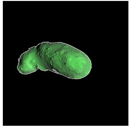
Figure 528: ST_2450874726_v.fits
