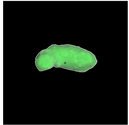
Figure 195: ST_2414830788_v.fits
