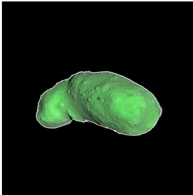
Figure 269: ST_2418871275_v.fits
