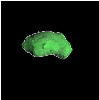
Figure 521: ST_2447767879_v.fits
