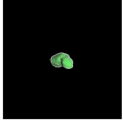
Figure 84: ST_2395637963_v.fits
