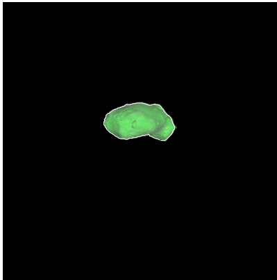
Figure 107: ST_2403064093_v.fits
