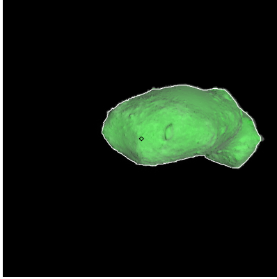
Figure 362: ST_2422600548_v.fits
