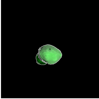
Figure 190: ST_2413033582_v.fits
