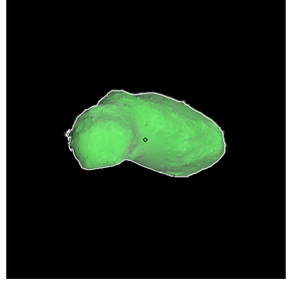
Figure 426: ST_2423296901_v.fits
