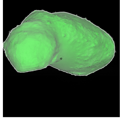
Figure 597: ST_2498724478_v.fits
