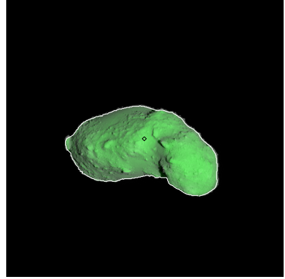
Figure 507: ST_2426409837_v.fits
