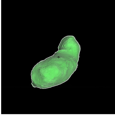
Figure 542: ST_2462068425_v.fits
