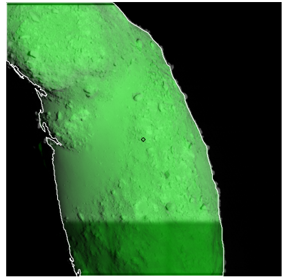
Figure 564: ST_2474846738_v.fits
