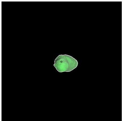
Figure 18: ST_2385718087_v.fits
