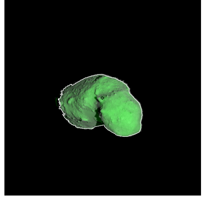
Figure 498: ST_2426336096_v.fits
