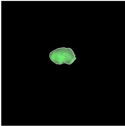
Figure 112: ST_2403131303_v.fits
