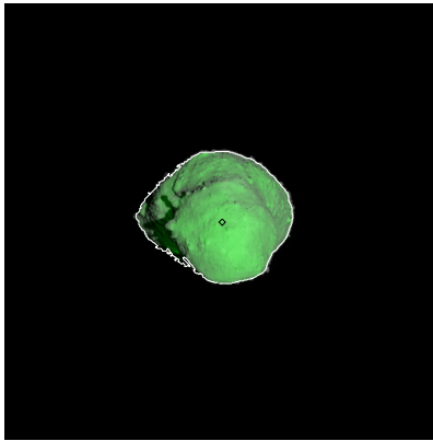
Figure 446: ST_2423460670_v.fits
