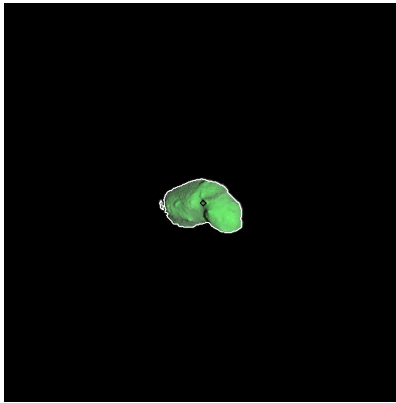
Figure 86: ST_2395653317_v.fits
