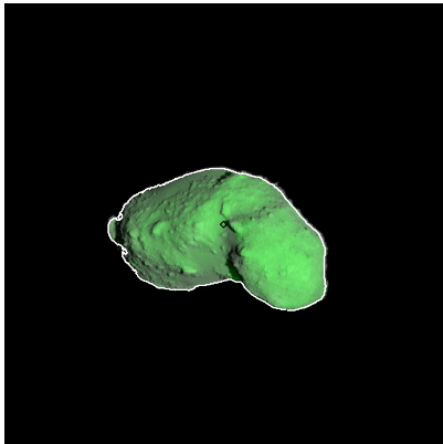
Figure 502: ST_2426368862_v.fits
