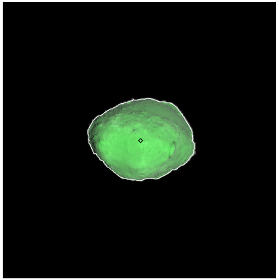
Figure 464: ST_2424116014_v.fits
