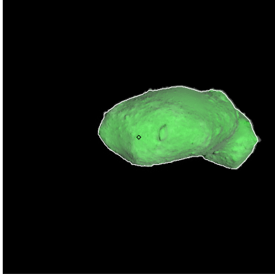
Figure 361: ST_2422592356_v.fits
