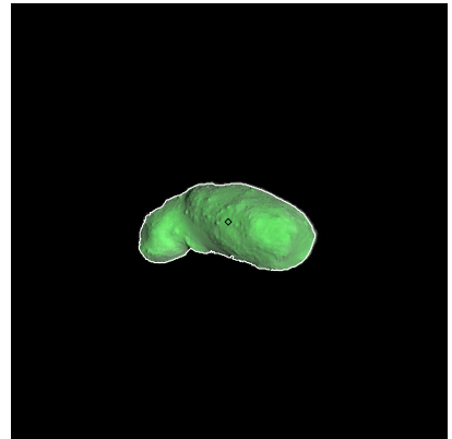
Figure 153: ST_2410406996_v.fits
