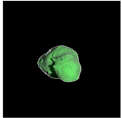
Figure 492: ST_2426286914_v.fits
