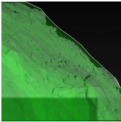
Figure 616: ST_2539467169_v.fits
