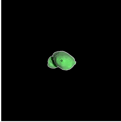
Figure 38: ST_2390750149_v.fits
