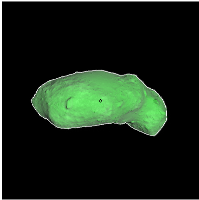
Figure 328: ST_2421126034_v.fits
