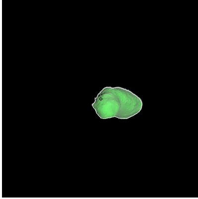
Figure 29: ST_2388484508_v.fits
