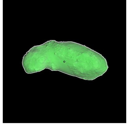
Figure 408: ST_2423149450_v.fits
