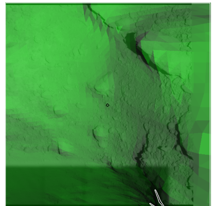
Figure 621: ST_2559003068_v.fits
