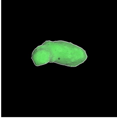
Figure 199: ST_2414861544_v.fits
