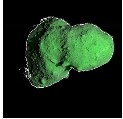
Figure 570: ST_2482160259_v.fits
