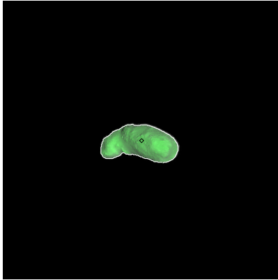
Figure 56: ST_2393672488_v.fits
