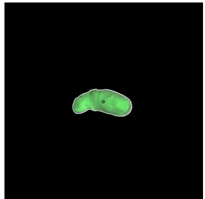
Figure 63: ST_2393726250_v.fits
