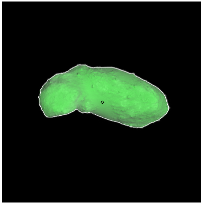
Figure 257: ST_2417620671_v.fits
