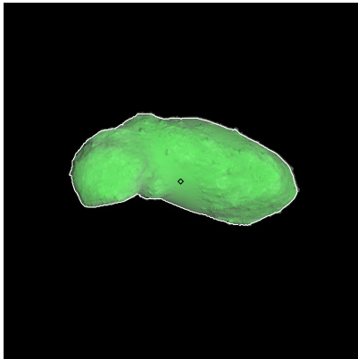
Figure 259: ST_2417636041_v.fits
