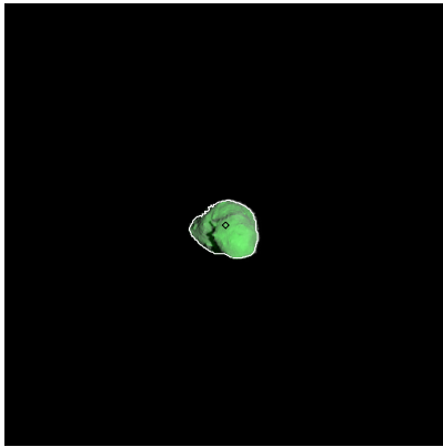
Figure 77: ST_2395576519_v.fits
