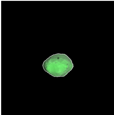
Figure 179: ST_2412949114_v.fits
