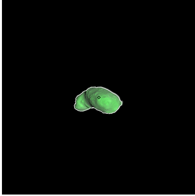
Figure 46: ST_2393595687_v.fits
