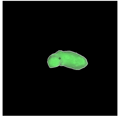
Figure 24: ST_2388340526_v.fits
