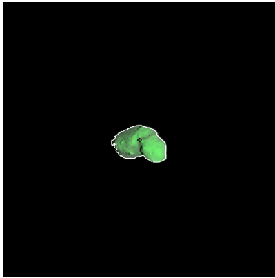
Figure 85: ST_2395645632_v.fits
