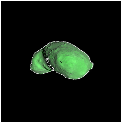
Figure 484: ST_2424279895_v.fits
