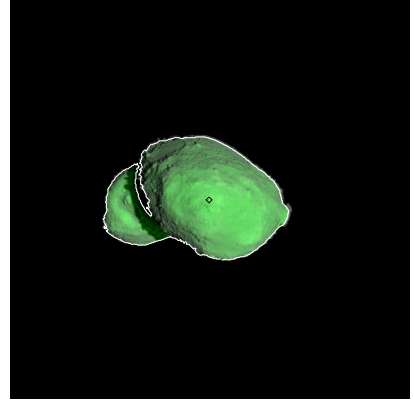
Figure 480: ST_2424247128_v.fits
