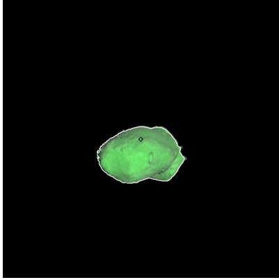
Figure 172: ST_2412895352_v.fits
