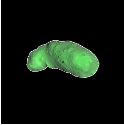
Figure 227: ST_2417390237_v.fits
