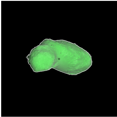
Figure 427: ST_2423305060_v.fits
