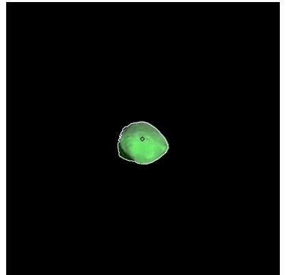
Figure 36: ST_2390692543_v.fits
