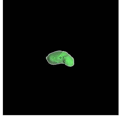
Figure 93: ST_2395707079_v.fits
