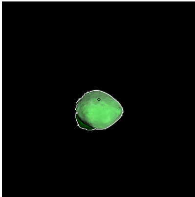
Figure 187: ST_2413010544_v.fits
