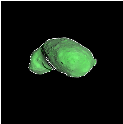
Figure 268: ST_2418859748_v.fits
