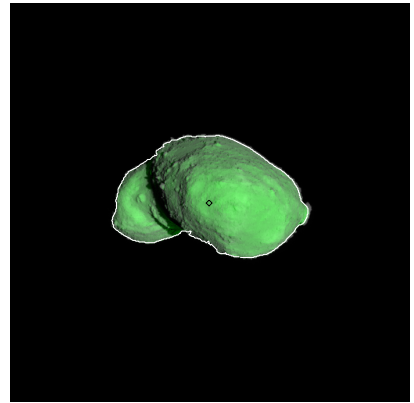
Figure 375: ST_2422870867_v.fits
