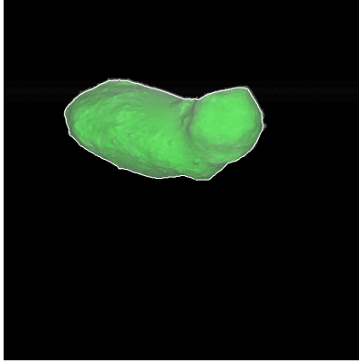
Figure 533: ST_2456824763_v.fits
