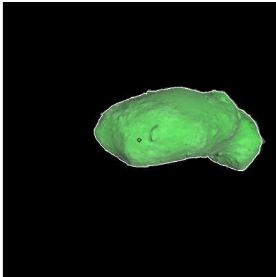
Figure 358: ST_2422567781_v.fits
