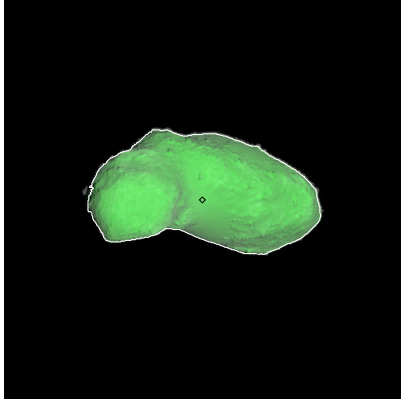
Figure 424: ST_2423280484_v.fits
