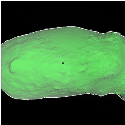
Figure 592: ST_2497841238_v.fits
