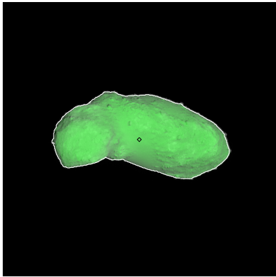
Figure 418: ST_2423231350_v.fits
