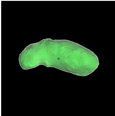
Figure 404: ST_2423116667_v.fits
