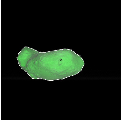
Figure 532: ST_2456125874_v.fits
