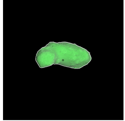
Figure 201: ST_2414876898_v.fits
