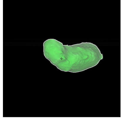
Figure 534: ST_2458536454_v.fits
