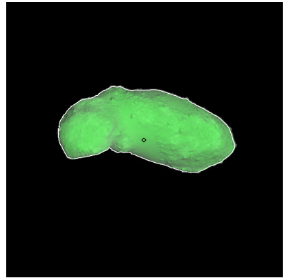
Figure 258: ST_2417628356_v.fits
