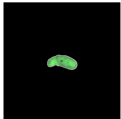
Figure 9: ST_2370315564_b.fits
