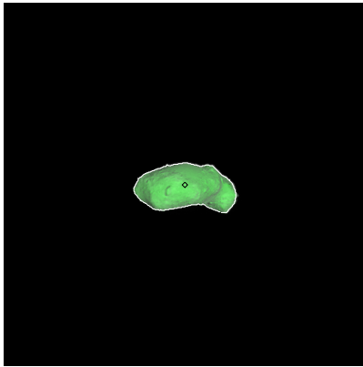
Figure 104: ST_2403016095_v.fits
