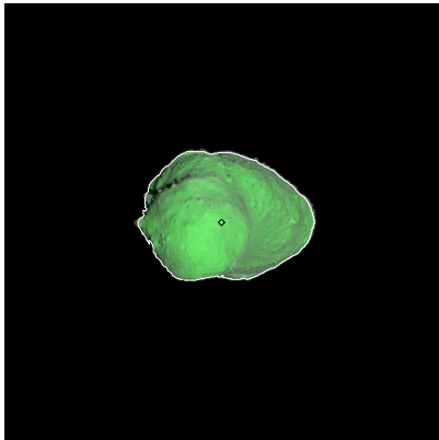
Figure 439: ST_2423403328_v.fits
