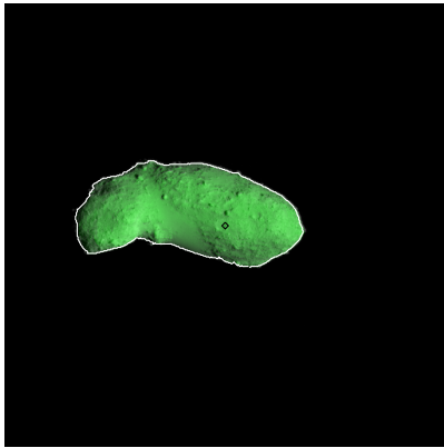
Figure 517: ST_2445692340_v.fits
