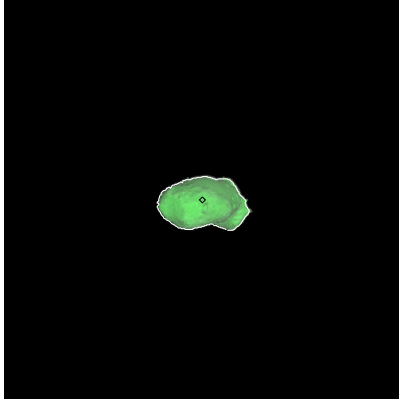
Figure 109: ST_2403102494_v.fits
