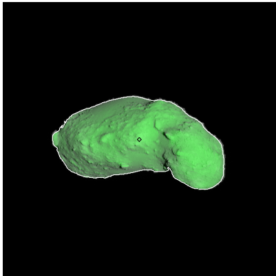
Figure 295: ST_2420855658_v.fits
