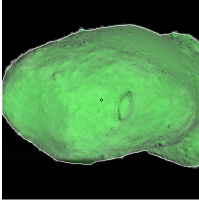
Figure 587: ST_2495230070_v.fits
