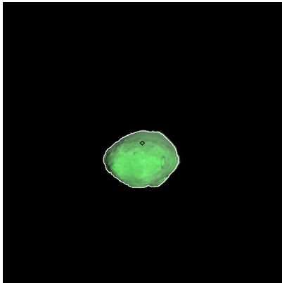
Figure 178: ST_2412941429_v.fits
