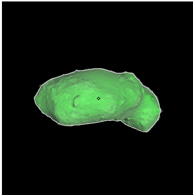
Figure 332: ST_2421158784_v.fits
