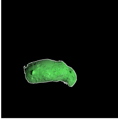
Figure 514: ST_2445001074_v.fits
