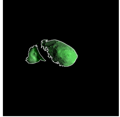
Figure 516: ST_2445206532_v.fits
