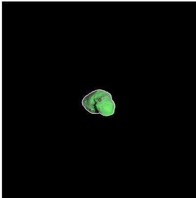
Figure 80: ST_2395599557_v.fits
