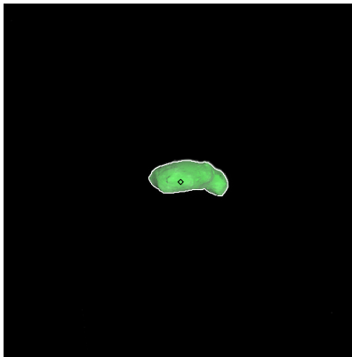
Figure 5: ST_2368071882_v.fits
