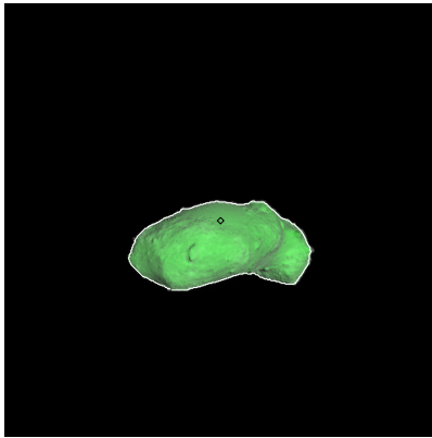
Figure 158: ST_2412787844_v.fits
