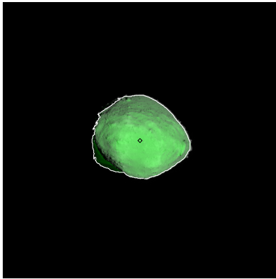
Figure 472: ST_2424181580_v.fits
