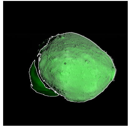
Figure 600: ST_2506540935_v.fits
