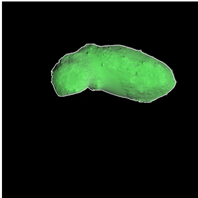
Figure 529: ST_2451105131_v.fits
