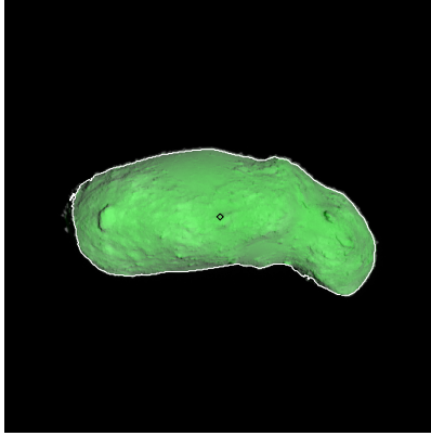
Figure 317: ST_2421035909_v.fits
