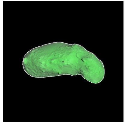
Figure 303: ST_2420921208_v.fits
