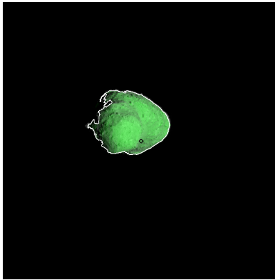
Figure 518: ST_2445698045_v.fits
