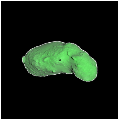
Figure 296: ST_2420863866_v.fits
