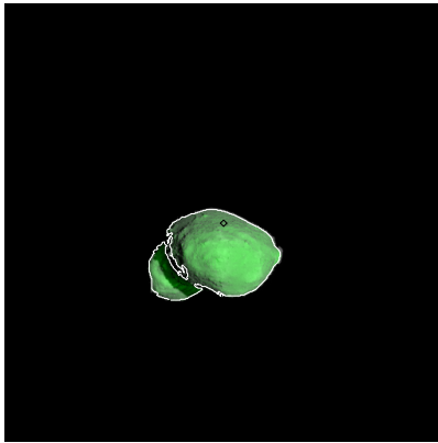
Figure 194: ST_2413064306_v.fits
