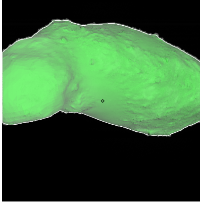
Figure 596: ST_2498647696_v.fits
