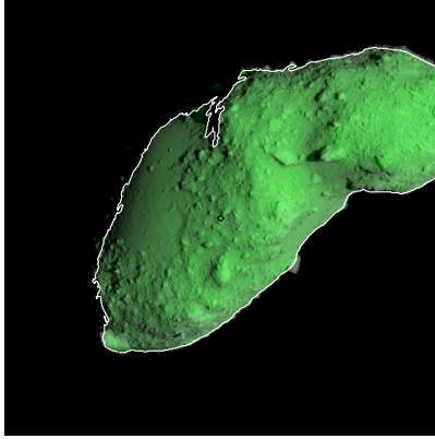
Figure 577: ST_2485860275_v.fits
