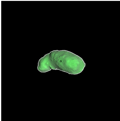
Figure 151: ST_2410391643_v.fits
