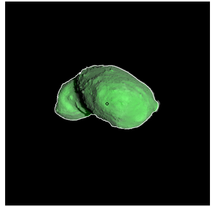
Figure 483: ST_2424271703_v.fits
