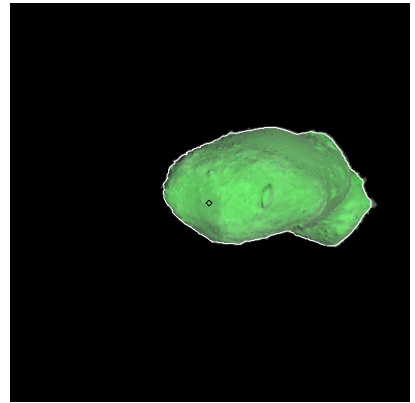
Figure 366: ST_2422633331_v.fits
