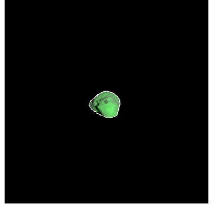
Figure 75: ST_2395561149_v.fits
