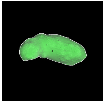
Figure 414: ST_2423198600_v.fits
