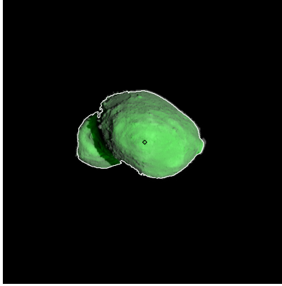
Figure 479: ST_2424238904_v.fits
