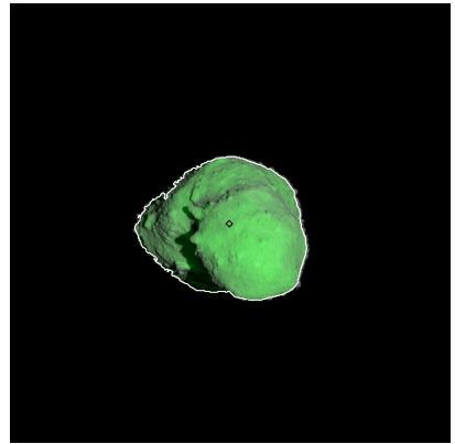
Figure 276: ST_2420699983_v.fits
