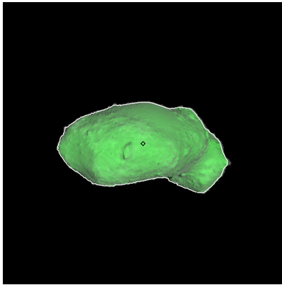
Figure 337: ST_2421199726_v.fits
