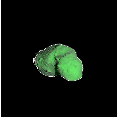
Figure 497: ST_2426327872_v.fits
