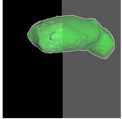
Figure 273: ST_2419737518_v.fits
