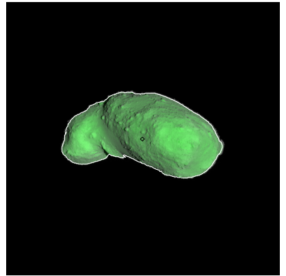
Figure 384: ST_2422944609_v.fits
