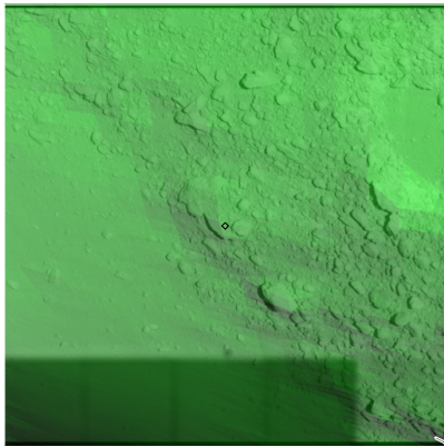
Figure 610: ST_2532629277_v.fits
