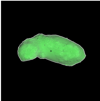
Figure 413: ST_2423190392_v.fits
