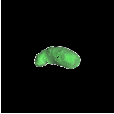
Figure 154: ST_2410414682_v.fits
