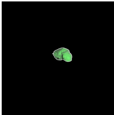
Figure 13: ST_2370554637_v.fits
