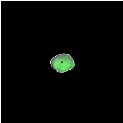
Figure 34: ST_2390634954_v.fits
