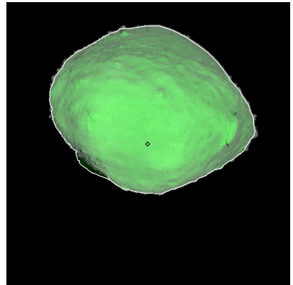
Figure 594: ST_2498167622_v.fits
