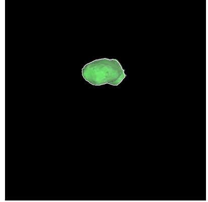
Figure 111: ST_2403121689_v.fits
