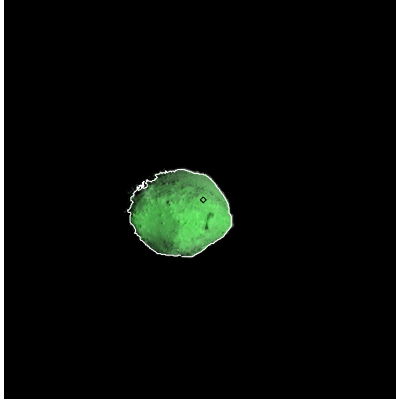
Figure 515: ST_2445006811_v.fits
