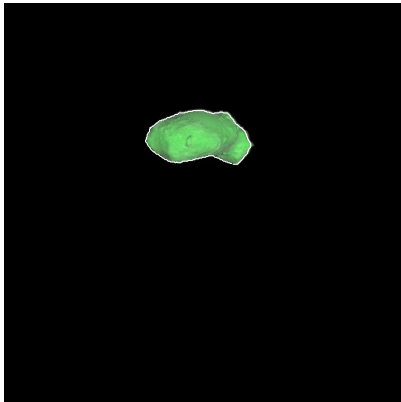
Figure 106: ST_2403054496_v.fits
