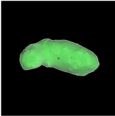
Figure 410: ST_2423165817_v.fits
