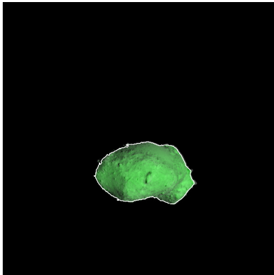
Figure 512: ST_2444259813_v.fits
