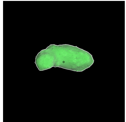
Figure 198: ST_2414853859_v.fits
