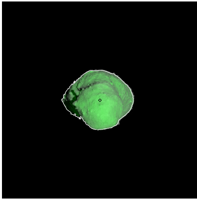
Figure 445: ST_2423452462_v.fits
