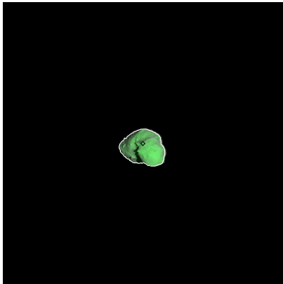
Figure 79: ST_2395591873_v.fits
