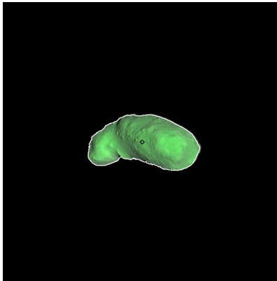
Figure 152: ST_2410399311_v.fits
