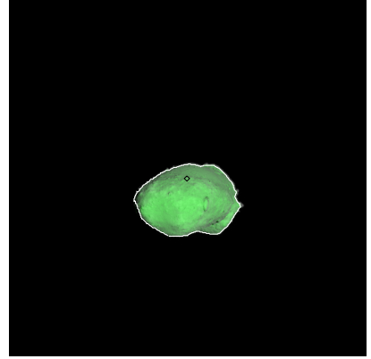
Figure 174: ST_2412910705_v.fits
