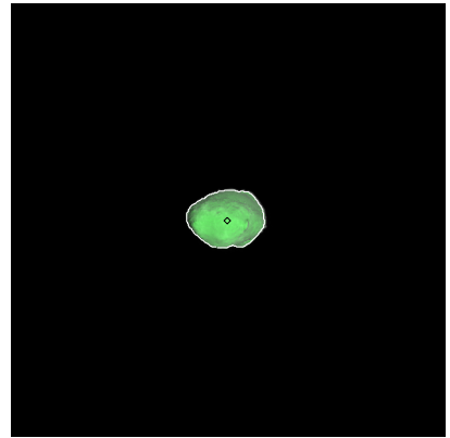
Figure 114: ST_2403169687_v.fits
