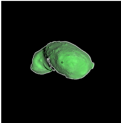
Figure 377: ST_2422887250_v.fits
