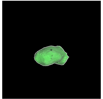
Figure 168: ST_2412864645_v.fits
