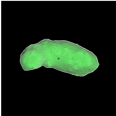
Figure 412: ST_2423182200_v.fits
