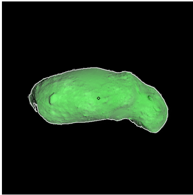
Figure 320: ST_2421060484_v.fits
