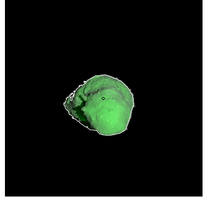
Figure 489: ST_2426262322_v.fits
