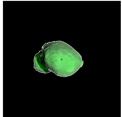
Figure 477: ST_242422537_v.fits
