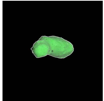
Figure 207: ST_2414922975_v.fits
