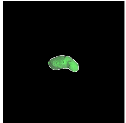
Figure 96: ST_2395730117_v.fits
