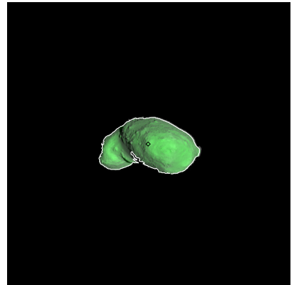
Figure 144: ST_2410337880_v.fits
