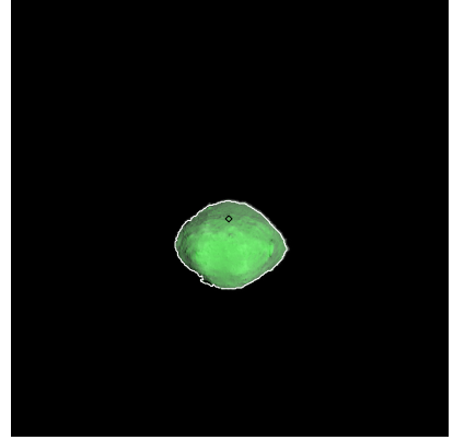
Figure 183: ST_2412979821_v.fits
