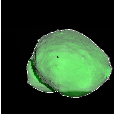
Figure 595: ST_2498206022_v.fits
