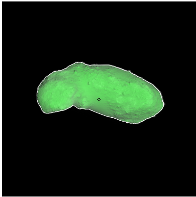
Figure 256: ST_2417613002_v.fits
