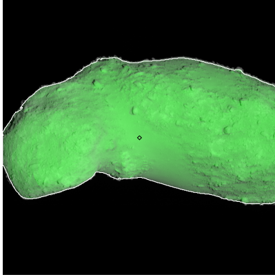
Figure 604: ST_2506925002_v.fits
