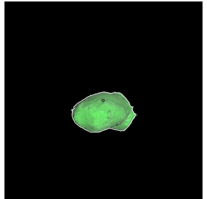
Figure 171: ST_2412887667_v.fits
