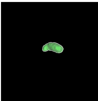
Figure 8: ST_2368576832_v.fits
