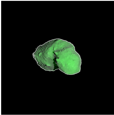
Figure 455: ST_2423534411_v.fits
