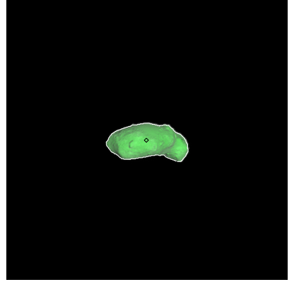
Figure 102: ST_2402996901_v.fits
