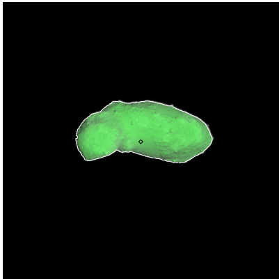
Figure 196: ST_2414838473_v.fits
