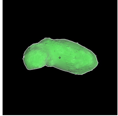
Figure 417: ST_2423223175_v.fits
