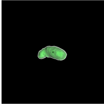
Figure 55: ST_2393664803_v.fits
