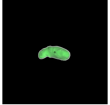
Figure 66: ST_2393749288_v.fits
