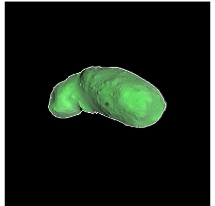
Figure 225: ST_2417374900_v.fits
