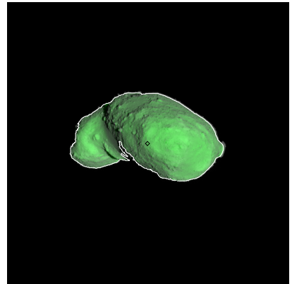
Figure 486: ST_2424296278_v.fits
