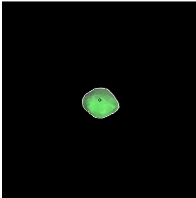
Figure 35: ST_2390663757_v.fits
