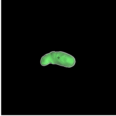
Figure 64: ST_2393733918_v.fits
