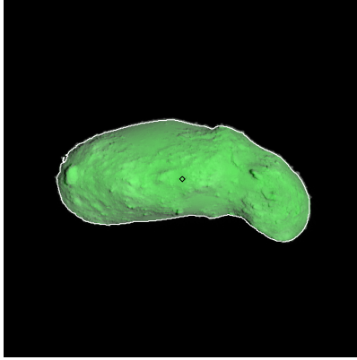
Figure 308: ST_2420962183_v.fits
