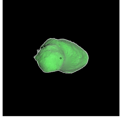
Figure 435: ST_2423370577_v.fits
