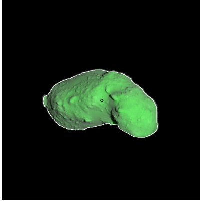
Figure 290: ST_2420814700_v.fits
