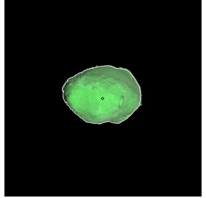
Figure 462: ST_2424099663_v.fits
