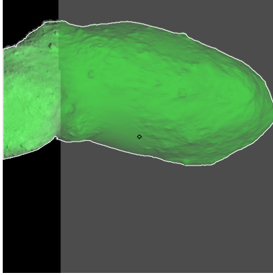
Figure 605: ST_2506963402_v.fits
