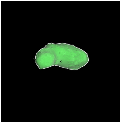
Figure 203: ST_2414892251_v.fits
