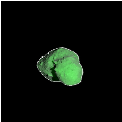
Figure 493: ST_2426295105_v.fits
