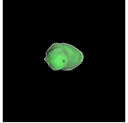
Figure 219: ST_2415015129_v.fits
