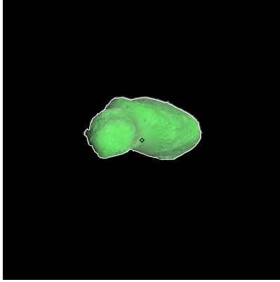
Figure 208: ST_2414930643_v.fits
