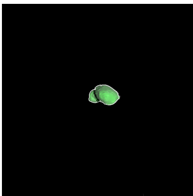
Figure 7: ST_2368423234_v.fits
