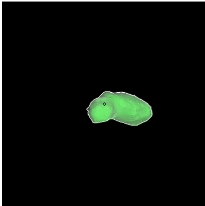
Figure 26: ST_2388398116_v.fits
