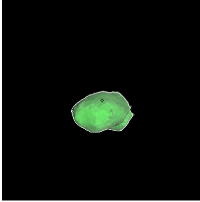
Figure 173: ST_2412903037_v.fits
