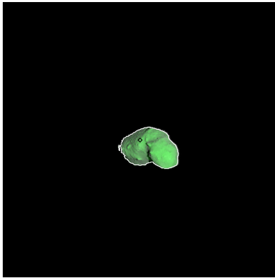
Figure 23: ST_2385864015_v.fits
