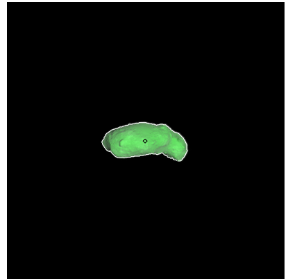
Figure 99: ST_2402948904_v.fits
