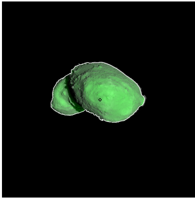
Figure 374: ST_2422862675_v.fits
