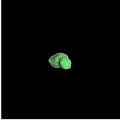
Figure 82: ST_2395622594_v.fits
