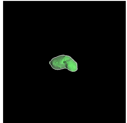
Figure 90: ST_2395684040_v.fits
