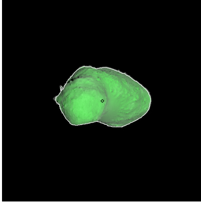
Figure 434: ST_2423362402_v.fits
