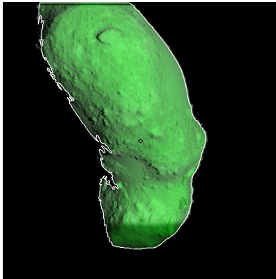
Figure 557: ST_2472776818_v.fits
