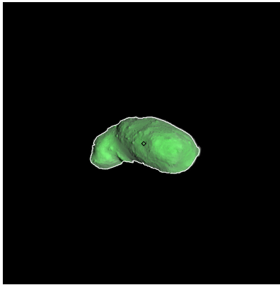
Figure 149: ST_2410376289_v.fits
