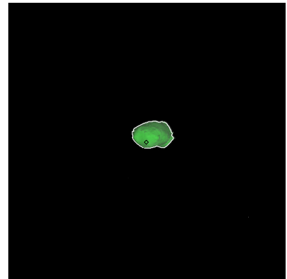
Figure 6: ST_2368246601_v.fits
