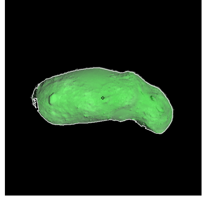
Figure 318: ST_2421044100_v.fits
