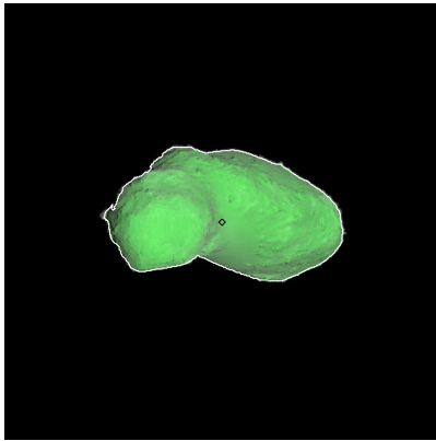
Figure 428: ST_2423313252_v.fits
