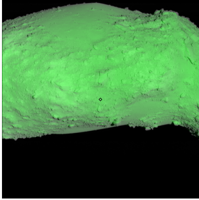
Figure 586: ST_2494991986_v.fits
