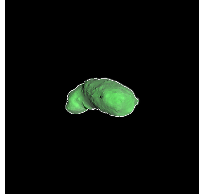
Figure 147: ST_2410360919_v.fits
