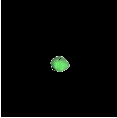
Figure 119: ST_2403236896_v.fits
