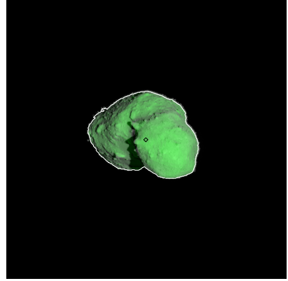
Figure 453: ST_2423518028_v.fits
