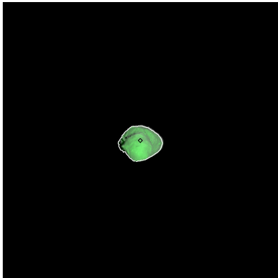
Figure 70: ST_2395522757_v.fits
