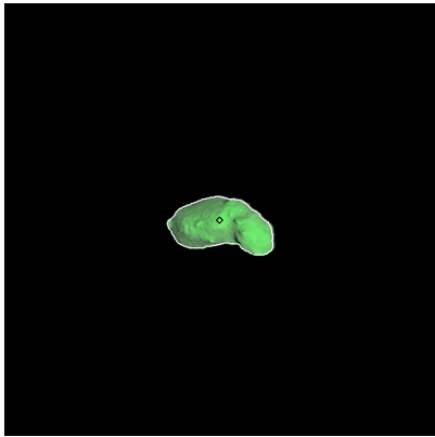
Figure 94: ST_2395714764_v.fits
