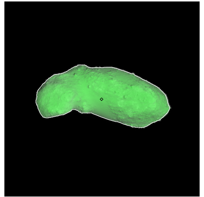
Figure 411: ST_2423174025_v.fits
