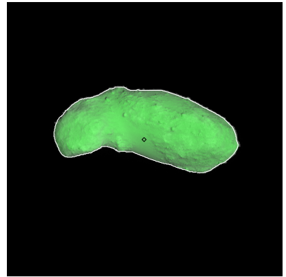
Figure 249: ST_2417559241_v.fits
