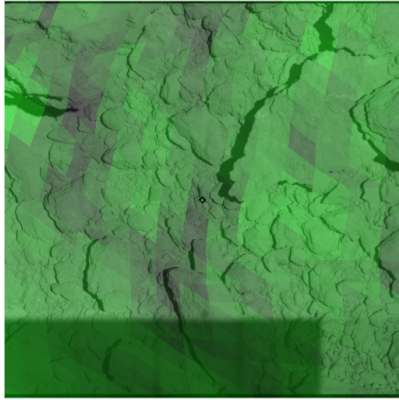
Figure 613: ST_2539437177_v.fits
