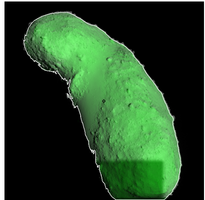
Figure 558: ST_2473314486_v.fits
