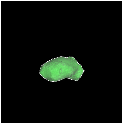
Figure 166: ST_2412849275_v.fits
