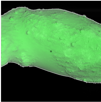
Figure 589: ST_2495748476_v.fits
