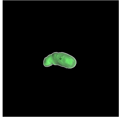
Figure 57: ST_2393680156_v.fits
