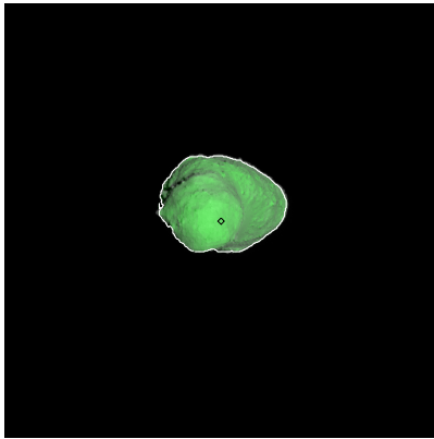
Figure 221: ST_2415030483_v.fits
