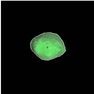
Figure 466: ST_2424132430_v.fits
