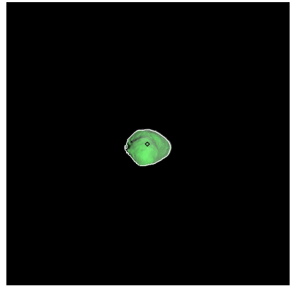
Figure 69: ST_2395515072_v.fits
