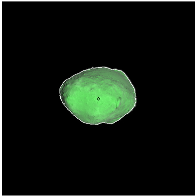
Figure 463: ST_2424107855_v.fits
