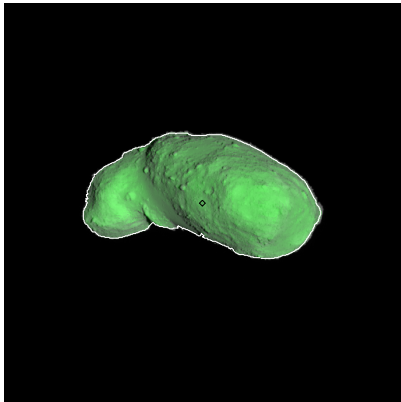
Figure 385: ST_2422952833_v.fits
