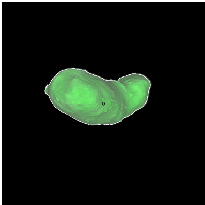
Figure 538: ST_2459278619_v.fits
