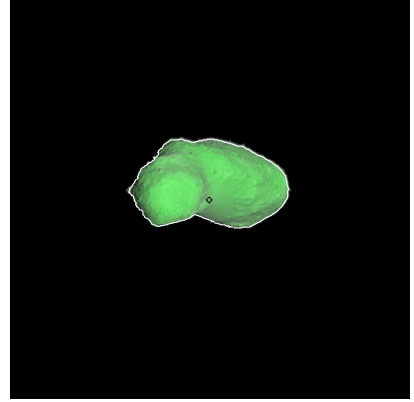
Figure 210: ST_2414946014_v.fits
