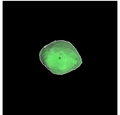
Figure 468: ST_2424148813_v.fits
