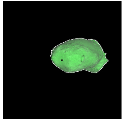
Figure 369: ST_2422657889_v.fits
