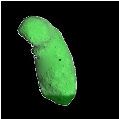
Figure 553: ST_2470681979_v.fits
