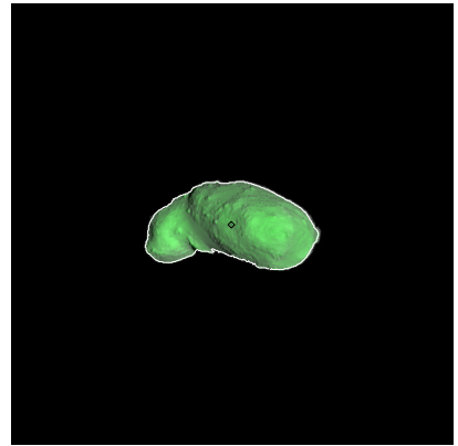
Figure 150: ST_2410383958_v.fits
