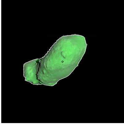
Figure 541: ST_2461722826_v.fits
