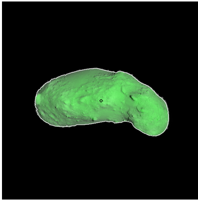
Figure 302: ST_2420913017_v.fits
