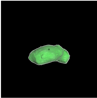
Figure 157: ST_2412780159_v.fits
