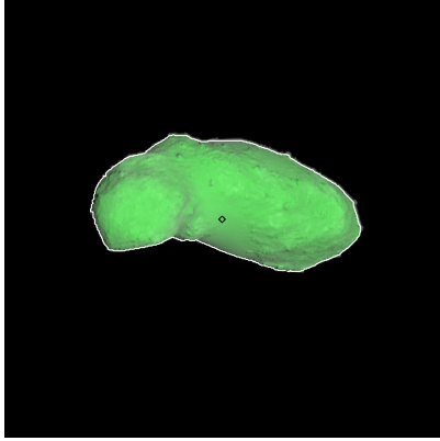
Figure 262: ST_2417659079_v.fits
