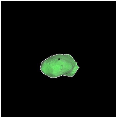
Figure 170: ST_2412879998_v.fits
