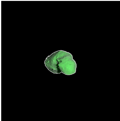
Figure 133: ST_2409562123_v.fits
