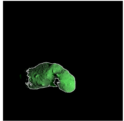
Figure 519: ST_2445901606_v.fits
