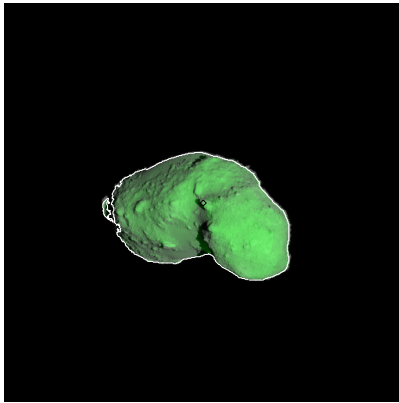
Figure 500: ST_2426352463_v.fits
