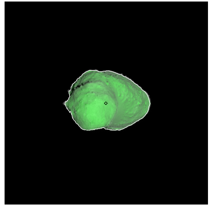
Figure 438: ST_2423395153_v.fits
