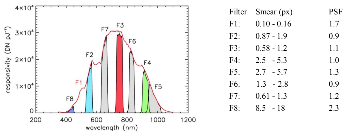
Figure 4-26. FC Filter wavelength response (left) and LAMO pixel smear and point spread functions (right). F1 is a broadband (clear) filter, sensitive in the wavelength interval from 400 to 1100 nm and peaking at 700 nm.
