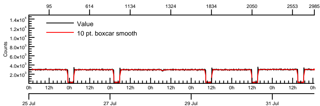
-Z phoswich CAT4 events
