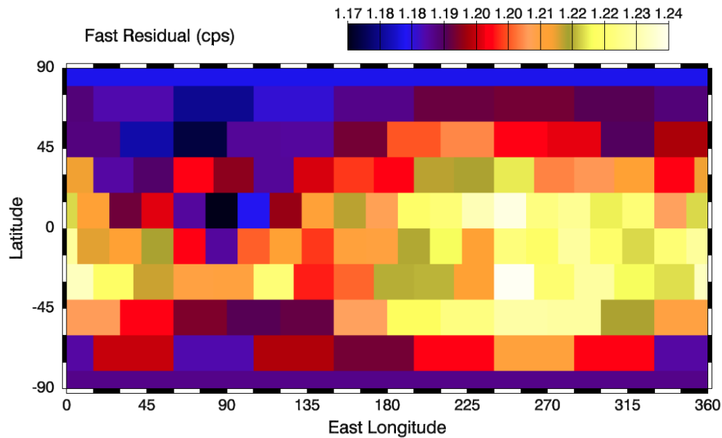
GRaND fast neutron residual data in Claudia double prime system.
