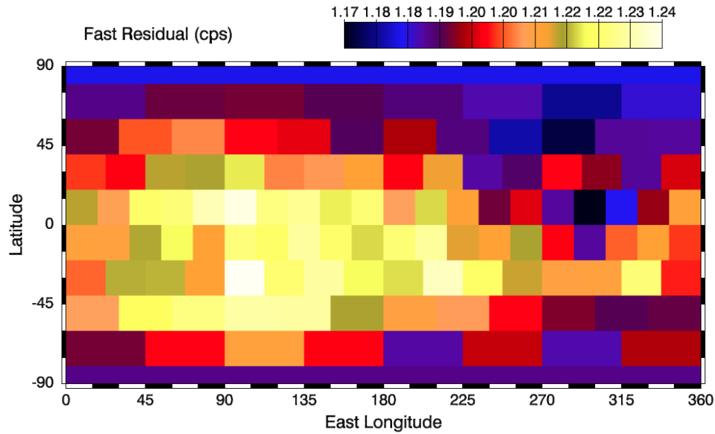
GRaND fast neutron residual map in Claudia system as given in Lawrence et al. (2013).
