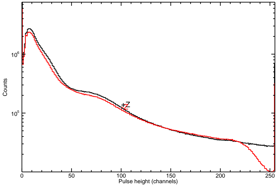
CAT1 histograms
