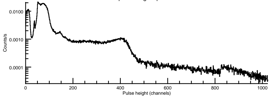
CAT10 pulse height spectrum: CZT0
