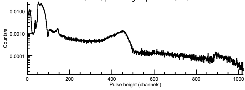
CAT10 pulse height spectrum: CZT10
