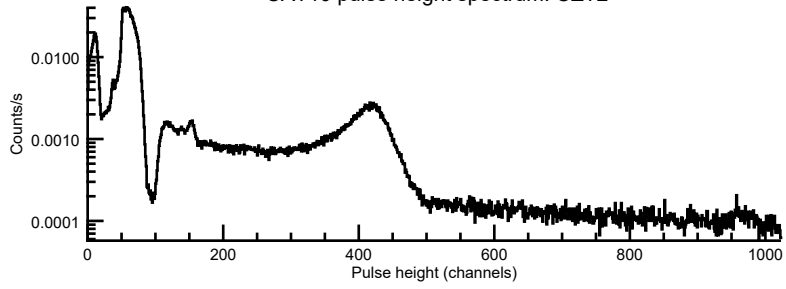
CAT10 pulse height spectrum: CZT8
