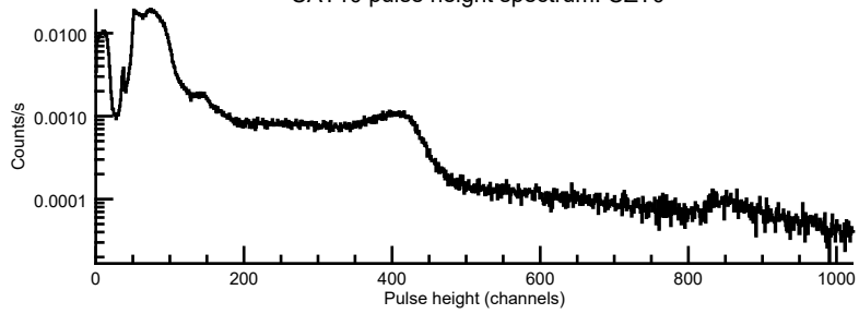
CAT10 pulse height spectrum: CZT0
