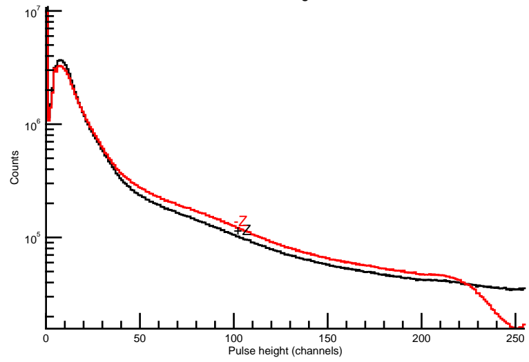
CAT1 histograms
