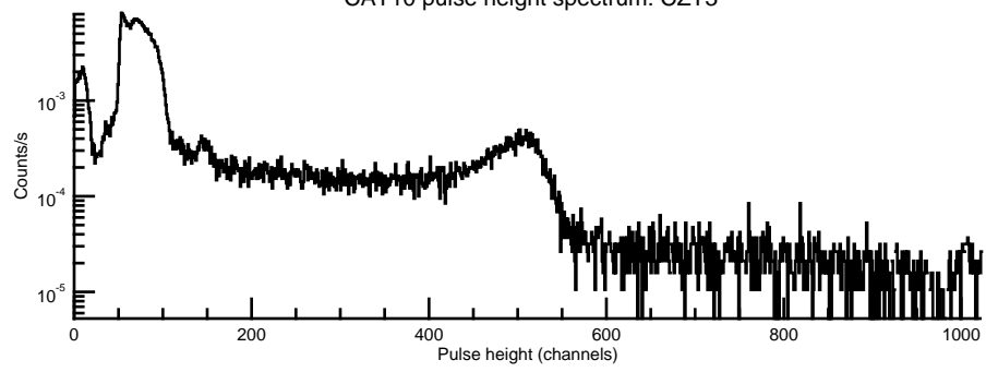
CAT10 pulse height spectrum: CZT1
