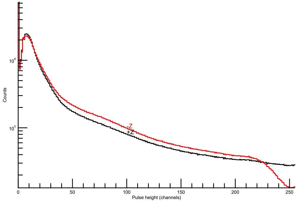
CAT1 histograms
